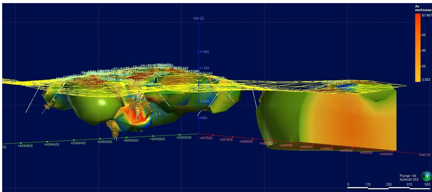
Diagram 1. Fran Gold Block Model (Smooth)
