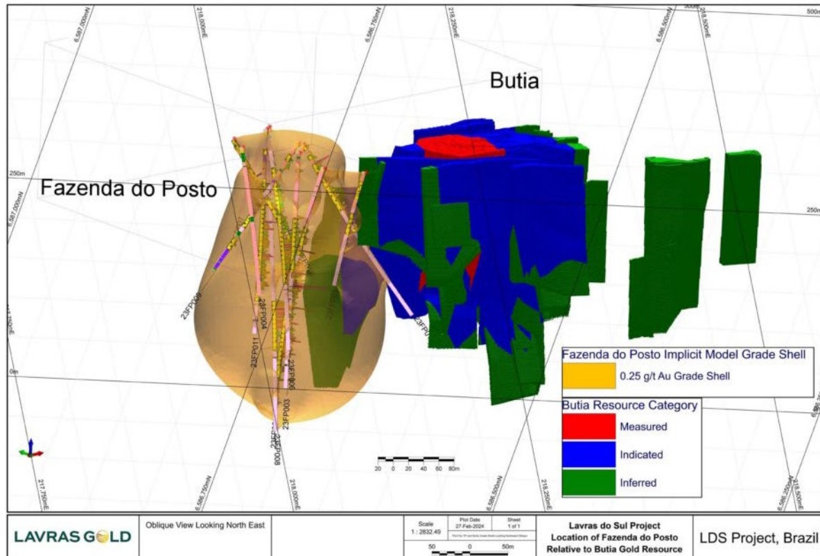
FIGURE 5: OUTLINE OF THE BUTIÁ GOLD DEPOSIT AND FAZENDA DO POSTO DISCOVERY (TOGETHER THE “BUTIÁ-FAZENDA PROJECT”)
