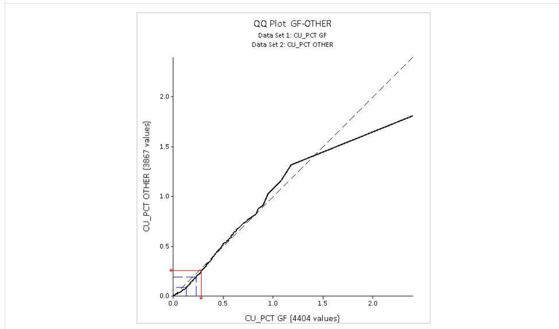
Figure 12-8 Great Fitzroy Mines Q-Q plot
