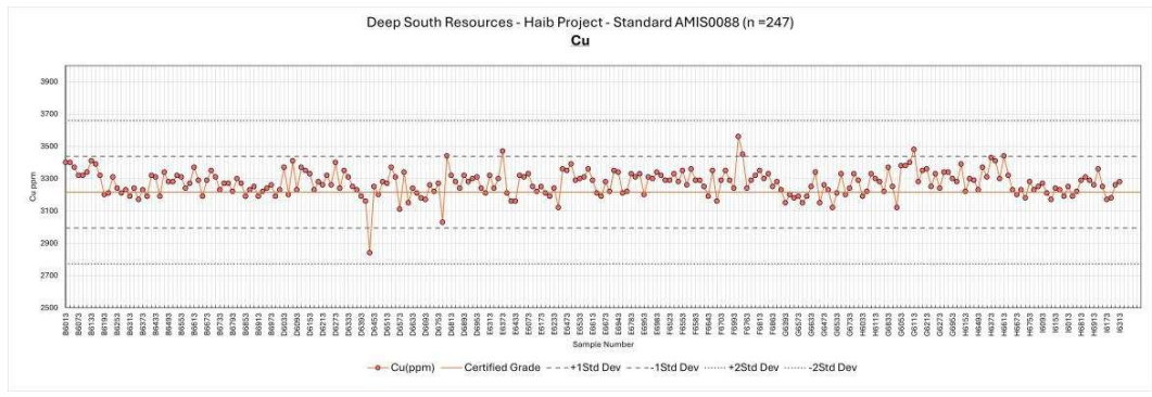
Figure 11-8 AMIS0088 control chart for Cu
