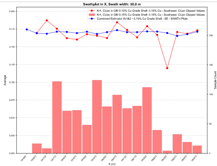
Figure 14-19 Swath plots for 0.15% Cu domain - SE zone
