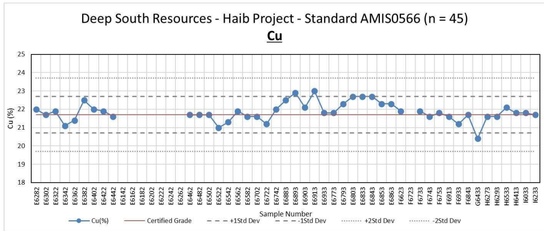
Figure 11-10 AMIS0566 control chart for Cu and Mo
