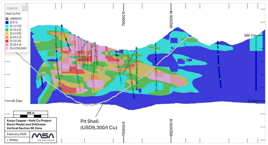
Figure 14-25 Section through Haib resource block model, drillholes and pit shell –SE Zone, view to the northwest
