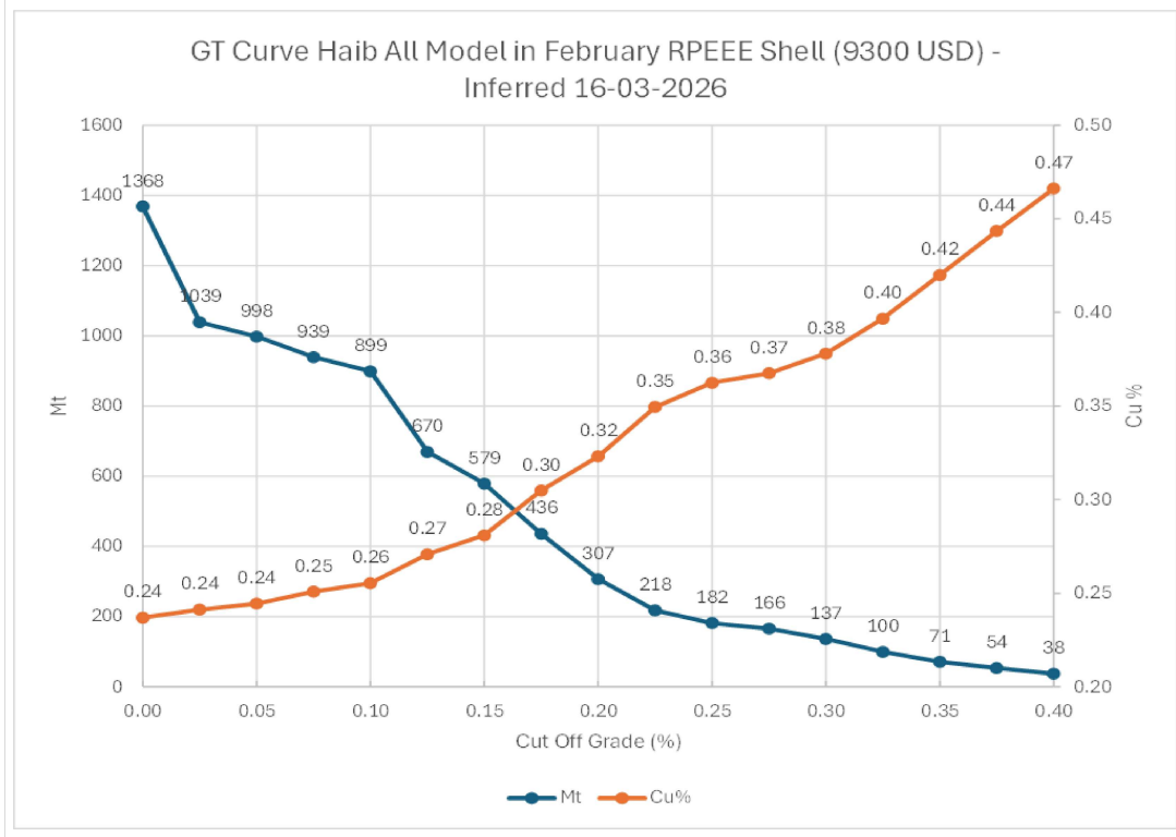
Figure 14-27 Grade-Tonnage Curves for Inferred Resource
