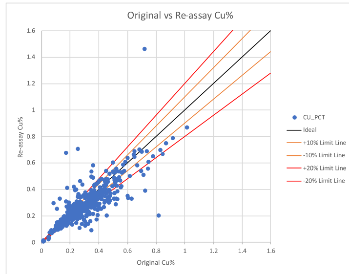
Figure 12-1 Scatterplot comparing RTZ original and Teck check sample results
