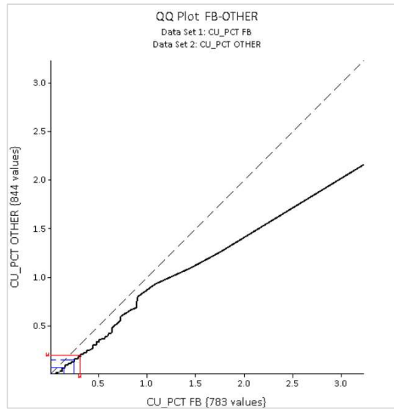
Figure 12-7 Falconbridge Q-Q plot
