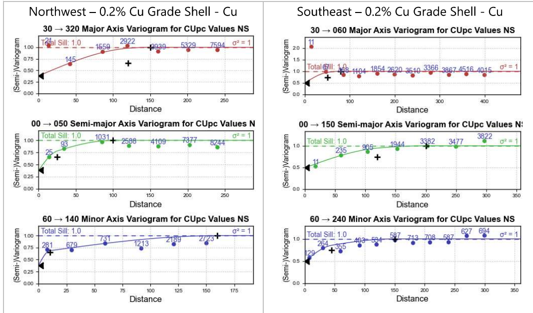
Figure 14-13 Semi-variograms for 0.2% Cu grade shells - Copper
