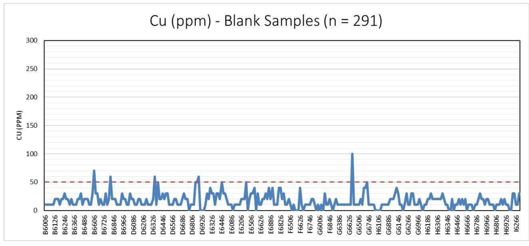
Figure 11-6 2021 - 2024 Blank control chart for Cu (ppm)
