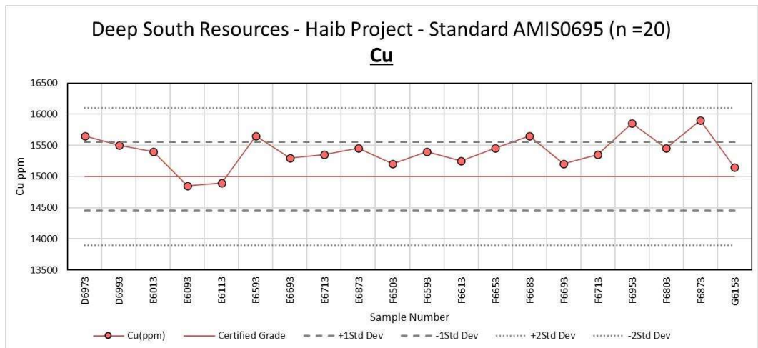
Figure 11-9 AMIS0695 control chart for Cu
