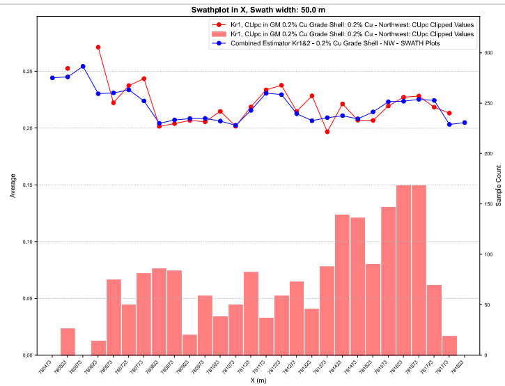
Figure 14-18 Swath plots for 0.2% Cu domain - NW zone
