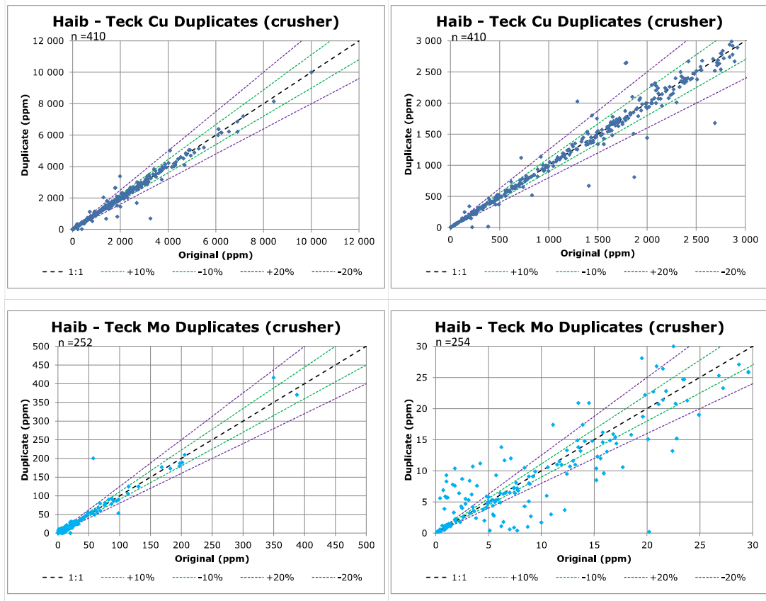
Figure 11-5 Teck coarse crush duplicates
