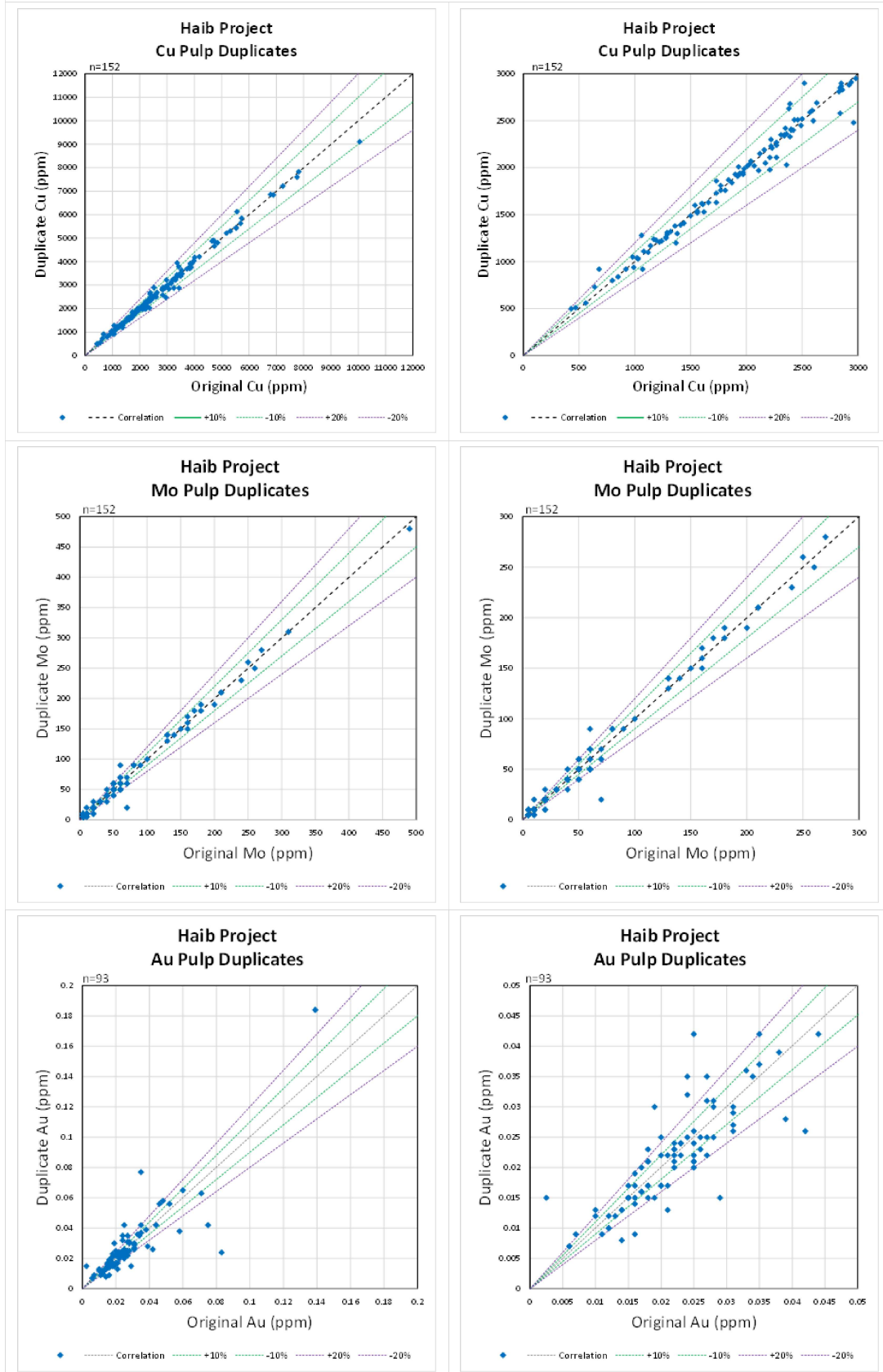
Figure 11-14 Scatterplot of Cu, Mo and Au pulp duplicate assays
