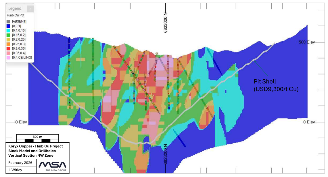
Figure 14-24 Section through Haib resource block model, drillholes and pit shell –NW Zone, view to the northwest
