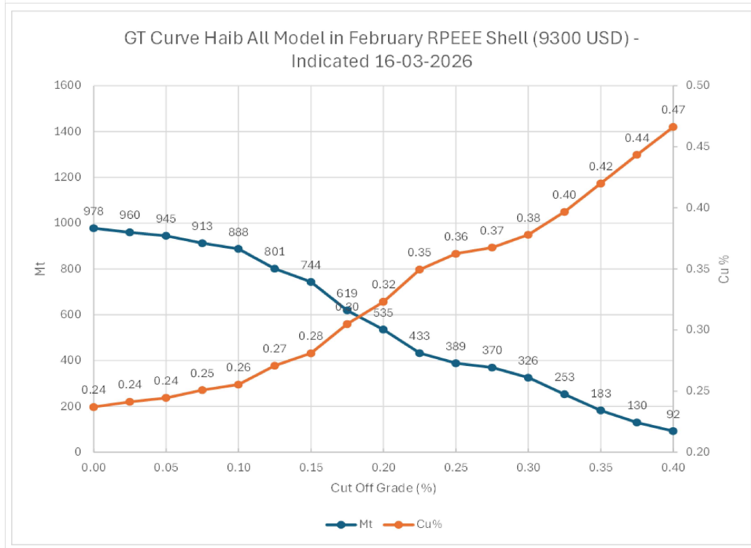
Figure 14-26 Grade-Tonnage Curves for Indicated Resource
