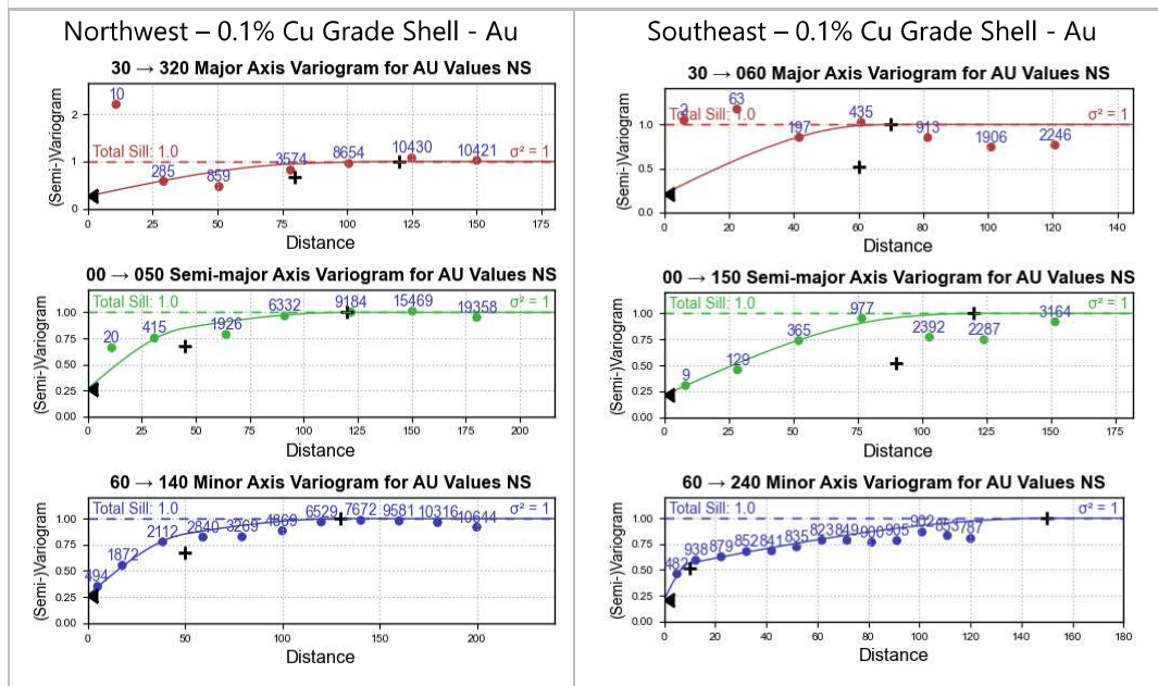
Figure 14-15 Semi-variograms for 0.1% Cu grade shells – Gold
