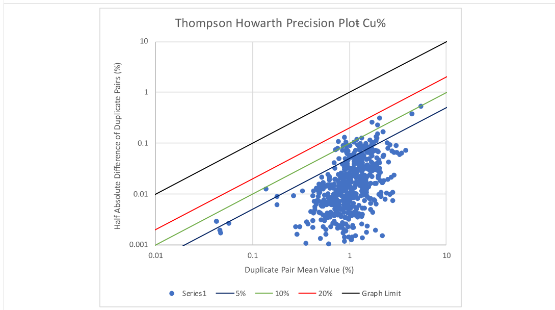
Figure 12-5 Thompson Howarth precision plot
