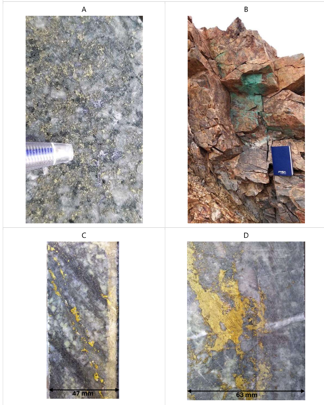
Figure 7-3 Examples of mineralisation at Haib
