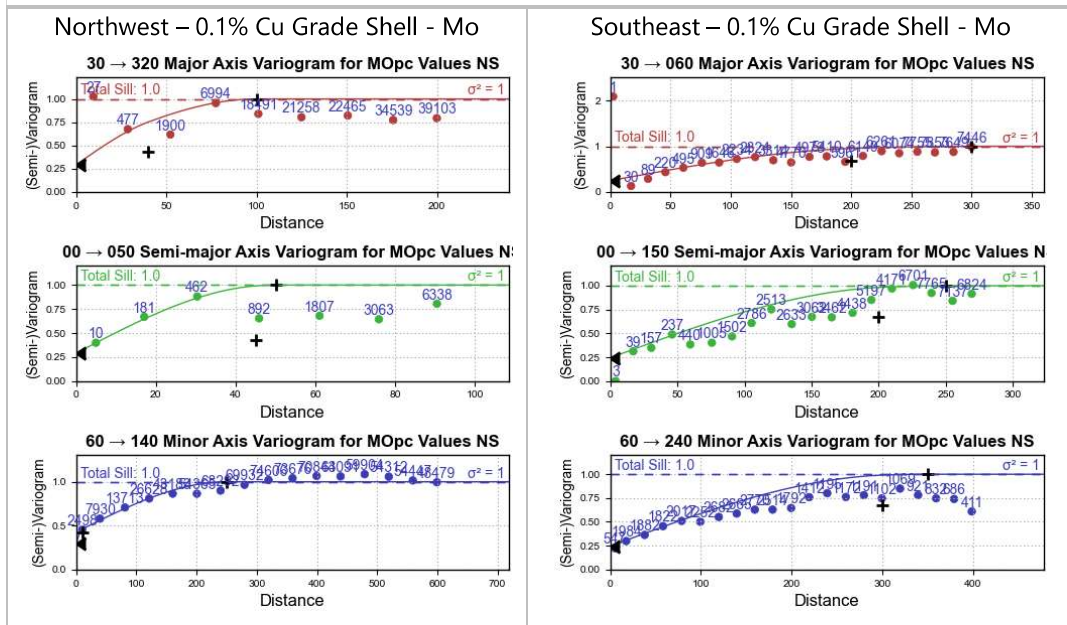
Figure 14-14 Semi-variograms for 0.1% Cu grade shells – Molybdenum
