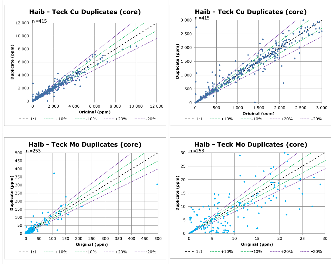
Figure 11-4 Teck quarter core duplicates
