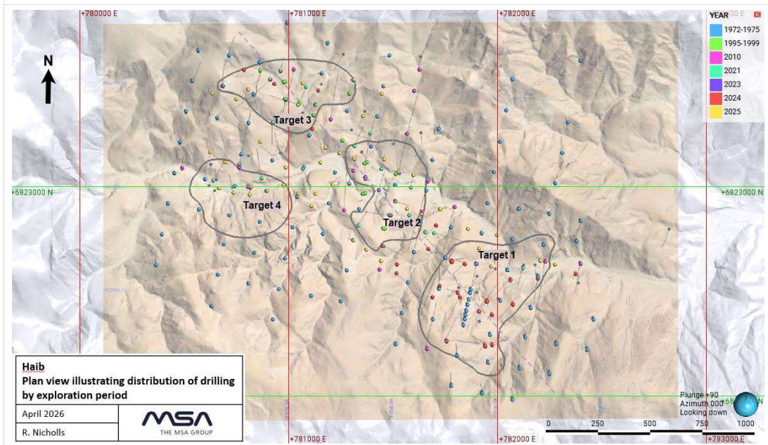
Figure 10-3 Drillhole collars by company
