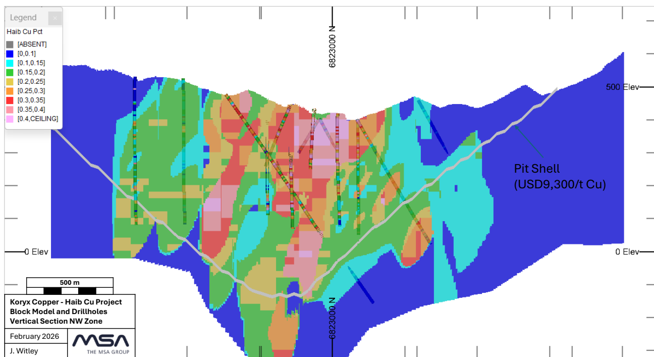
Figure 5. Section through Haib resource block model, drillholes and pit shell – NW Zone, view to the northwest
