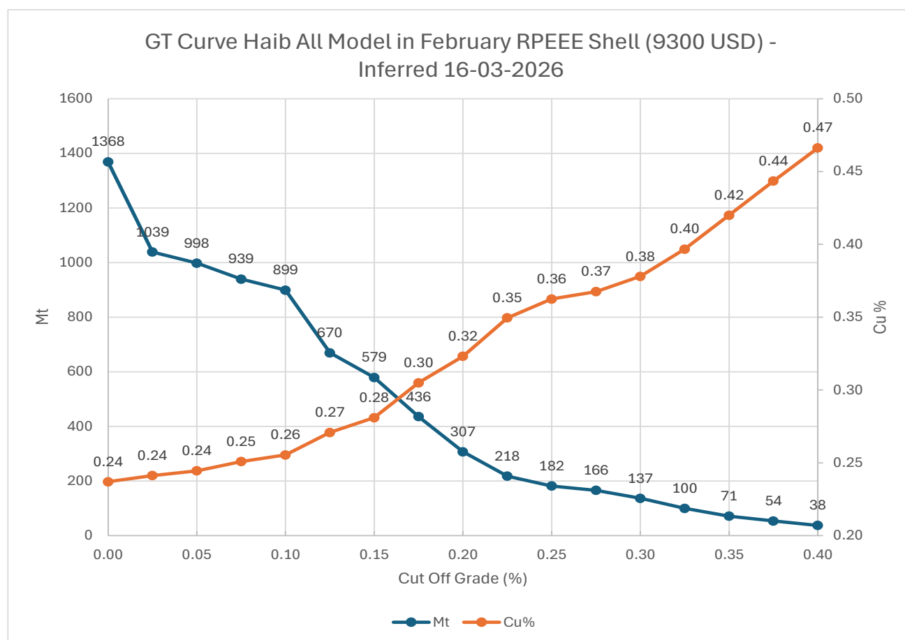
Figure 3. Grade-Tonnage Curve for Inferred Resources
