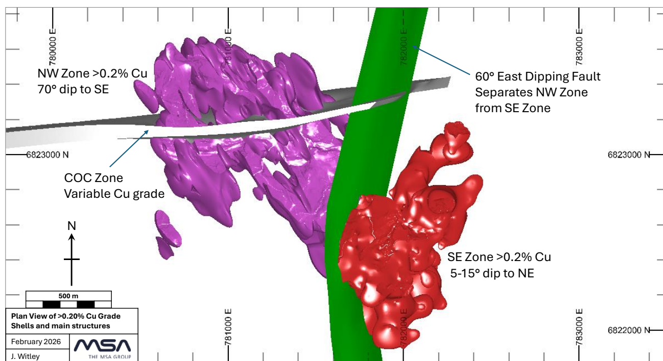
Figure 1. Plan view illustrating >0.2% Cu grade shells in the NW and SE zones and major structures
