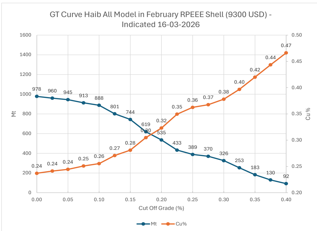
Figure 2. Grade-Tonnage Curve for Indicated Resources
