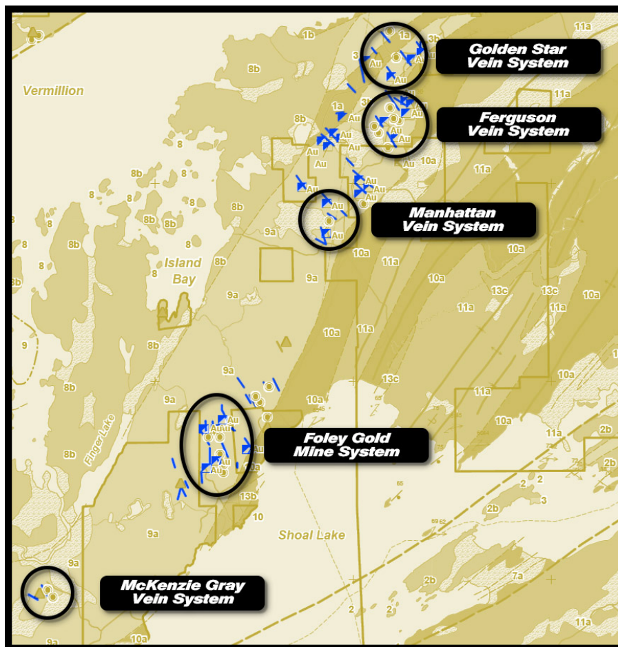
Figure 2 – Assorted Mine Centre Gold Vein Systems
