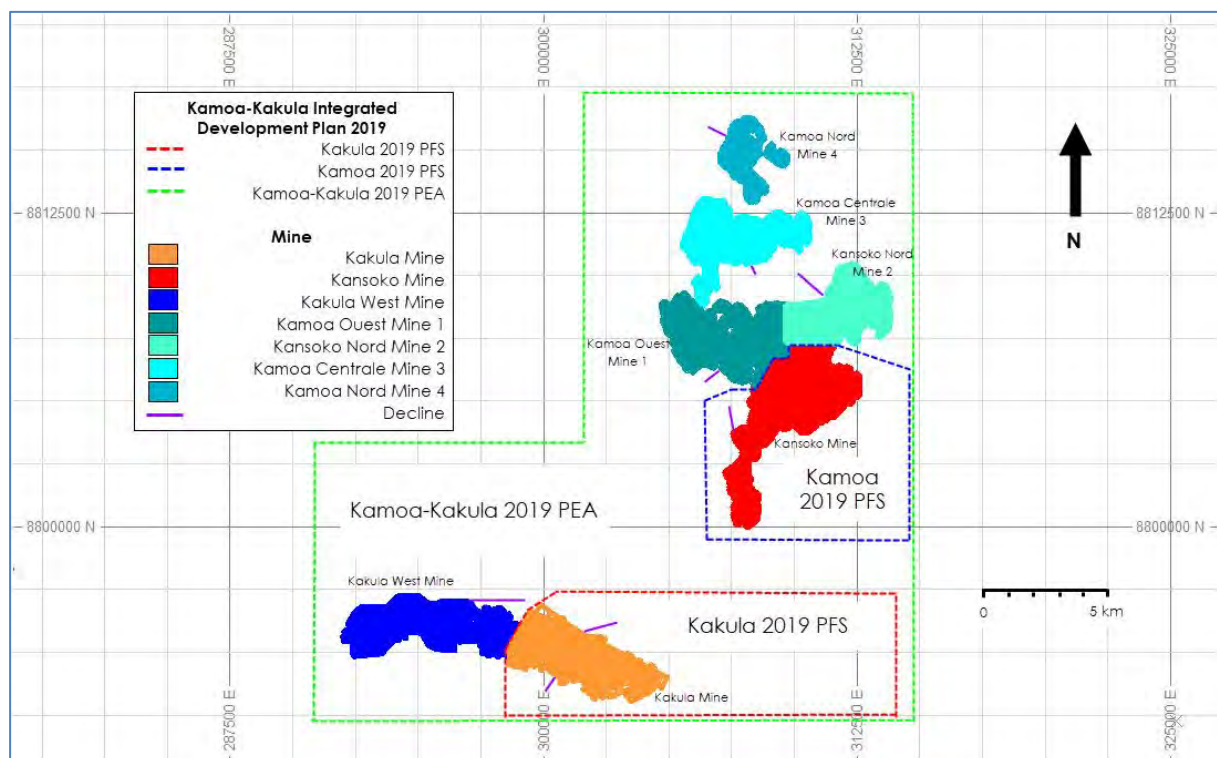
Figure 1.16 Kamoa-Kakula IDP19 Mining Locations
