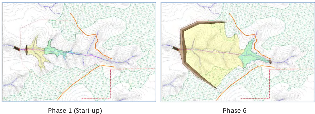
Figure 18.7 Containment Wall and Footprint Phasing
