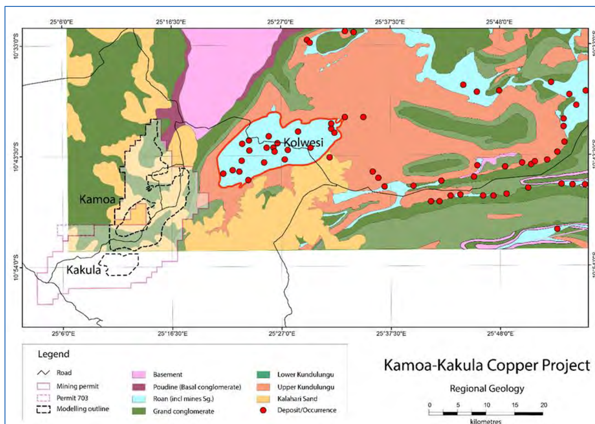
Figure 7.3 Location of the Kamoā-Kakula Project in Relation to the Regional Geology of the Kamoā and Kolwezi Area
