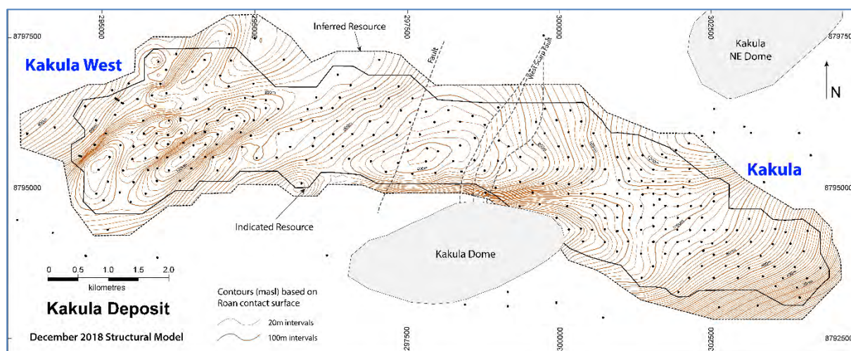
Figure 7.27 Structure Model for the Kakula Resource Area Showing Contours (masl) for the Ki1.1.1–R4.2 (Roan) contact
