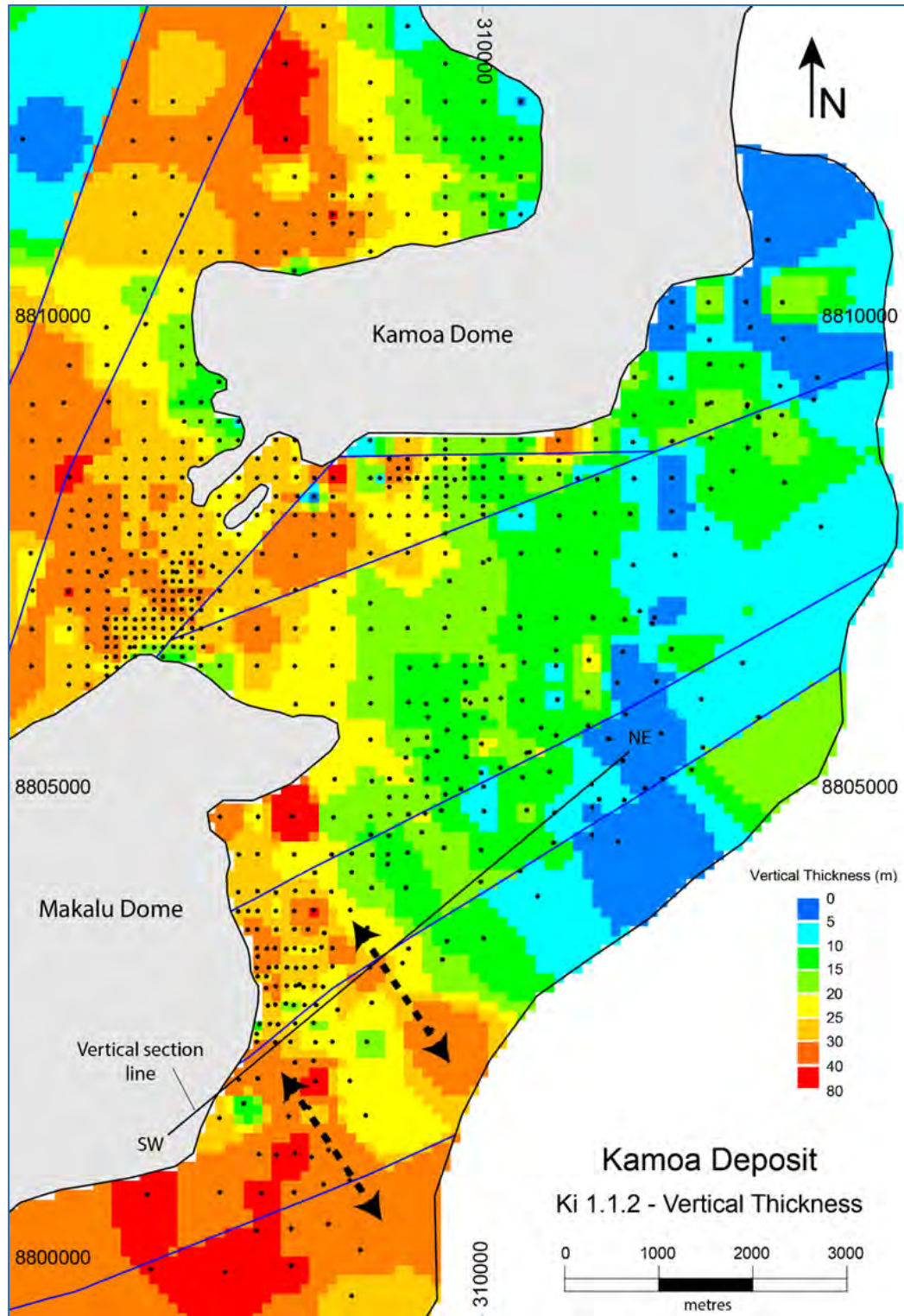
Figure 7.12 Ki 1.1.2 Vertical Thickness (KPS)
