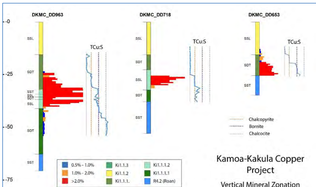
Figure 7.31 Examples from Three Drillholes from Kamoia of Vertical Mineral Zonation Evident Based on TCu:S Ratios
