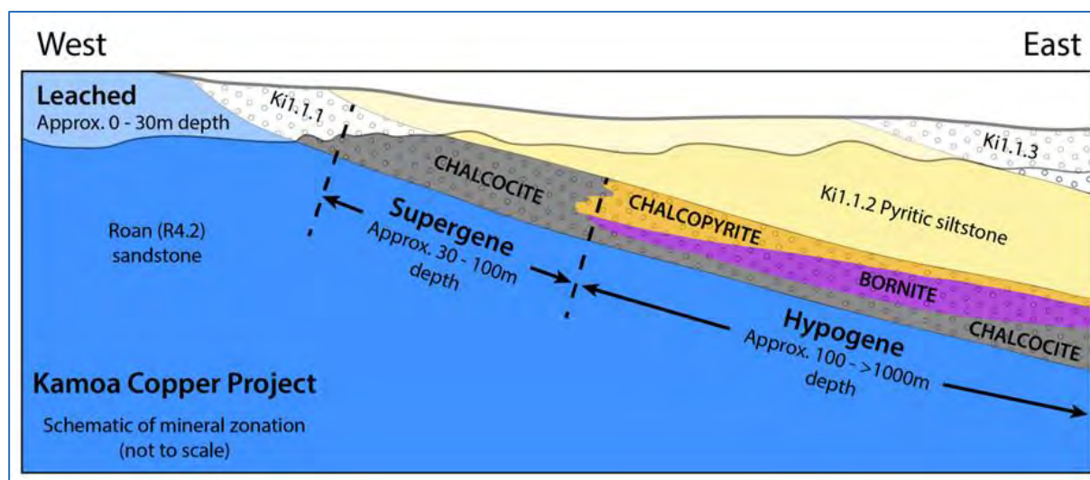
Figure 7.28 Schematic of Mineral Zonation at Kamoa
