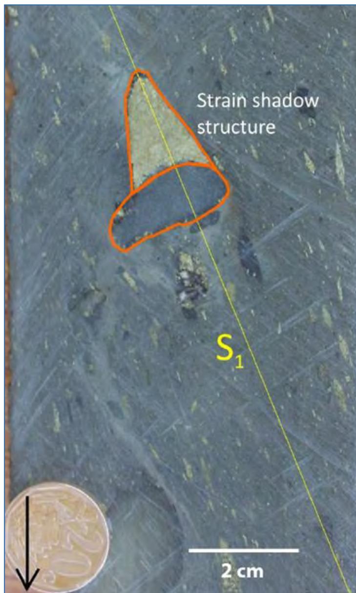
Figure provided by Ivanhoe, 2016. S_1 defines the orientation of the steep foliation.
