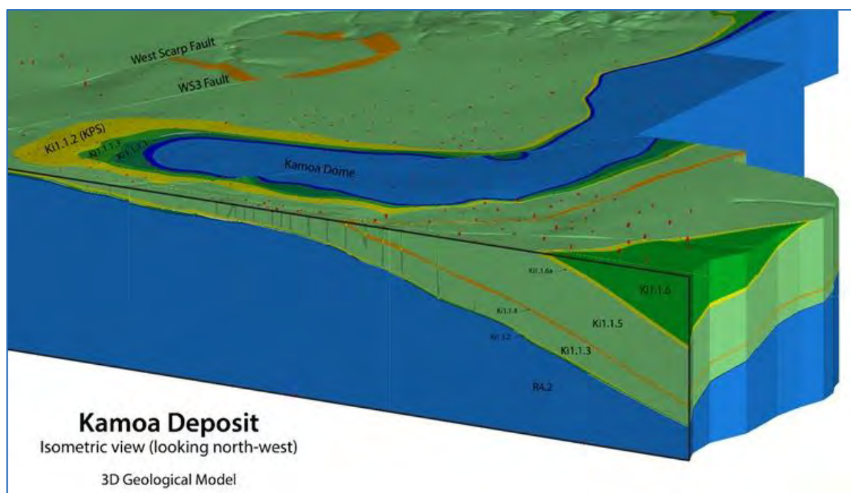
Figure 7.5 Isometric View of the Three-Dimensional Geological Model for Kamoā
