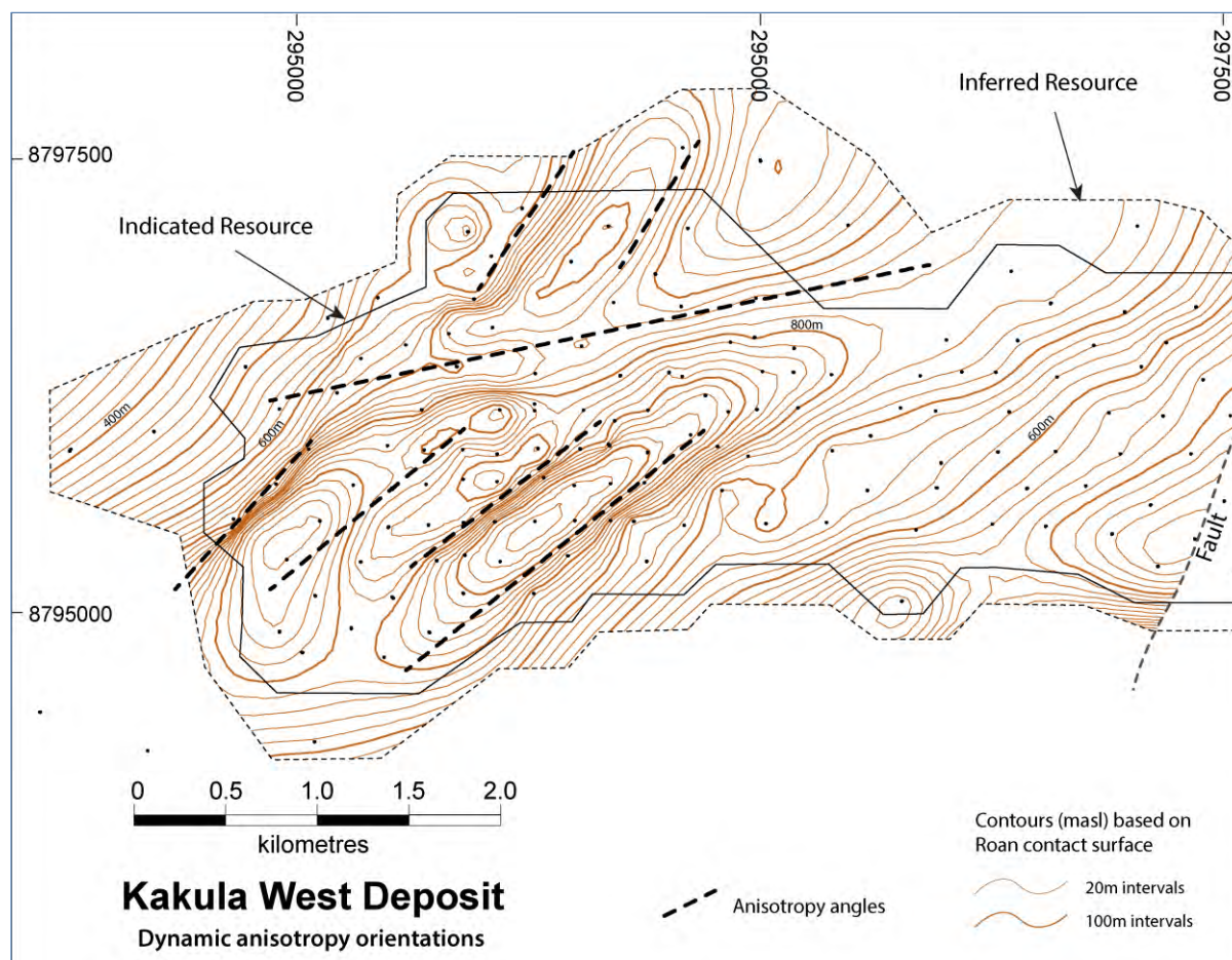
Figure 14.15 Kakula: Anisotropy Angles Used at Kaula West, Overlain on the Ki1.1.1-R4.2 (Roan) Contact
