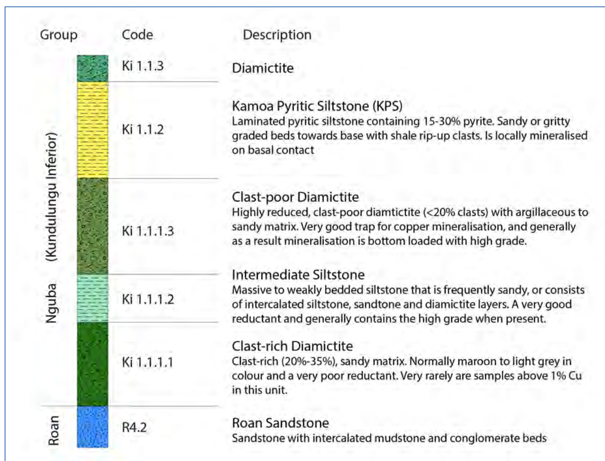
Figure 7.6 Local Stratigraphy for the Kamoia Deposit
