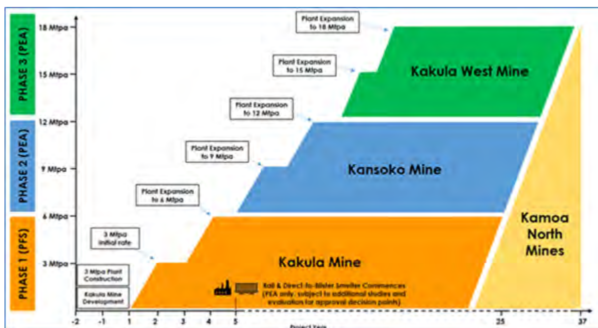
Figure 24.2 Kamo-a-Kakula IDP19 Long-Term Development Scenario
