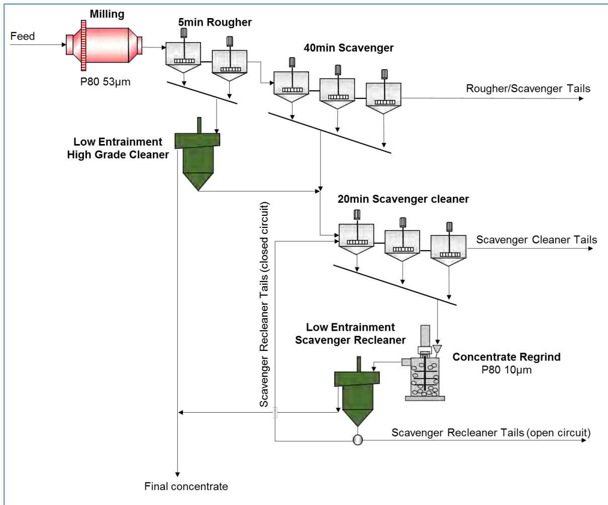
Figure 13.30 Kakula 2019 PFS Flow Sheet (Kamoa Copper SA, 2017)
