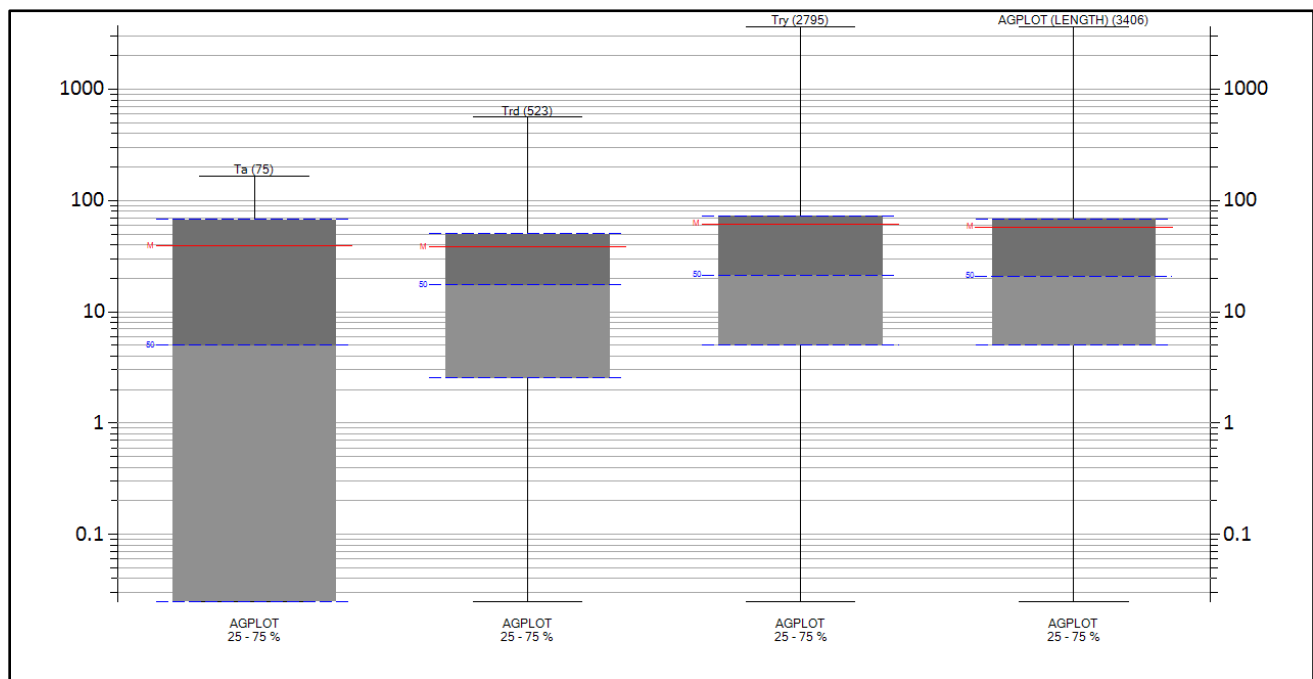
Figure 14-3 Silver box and whisker plot: Rock compositions
