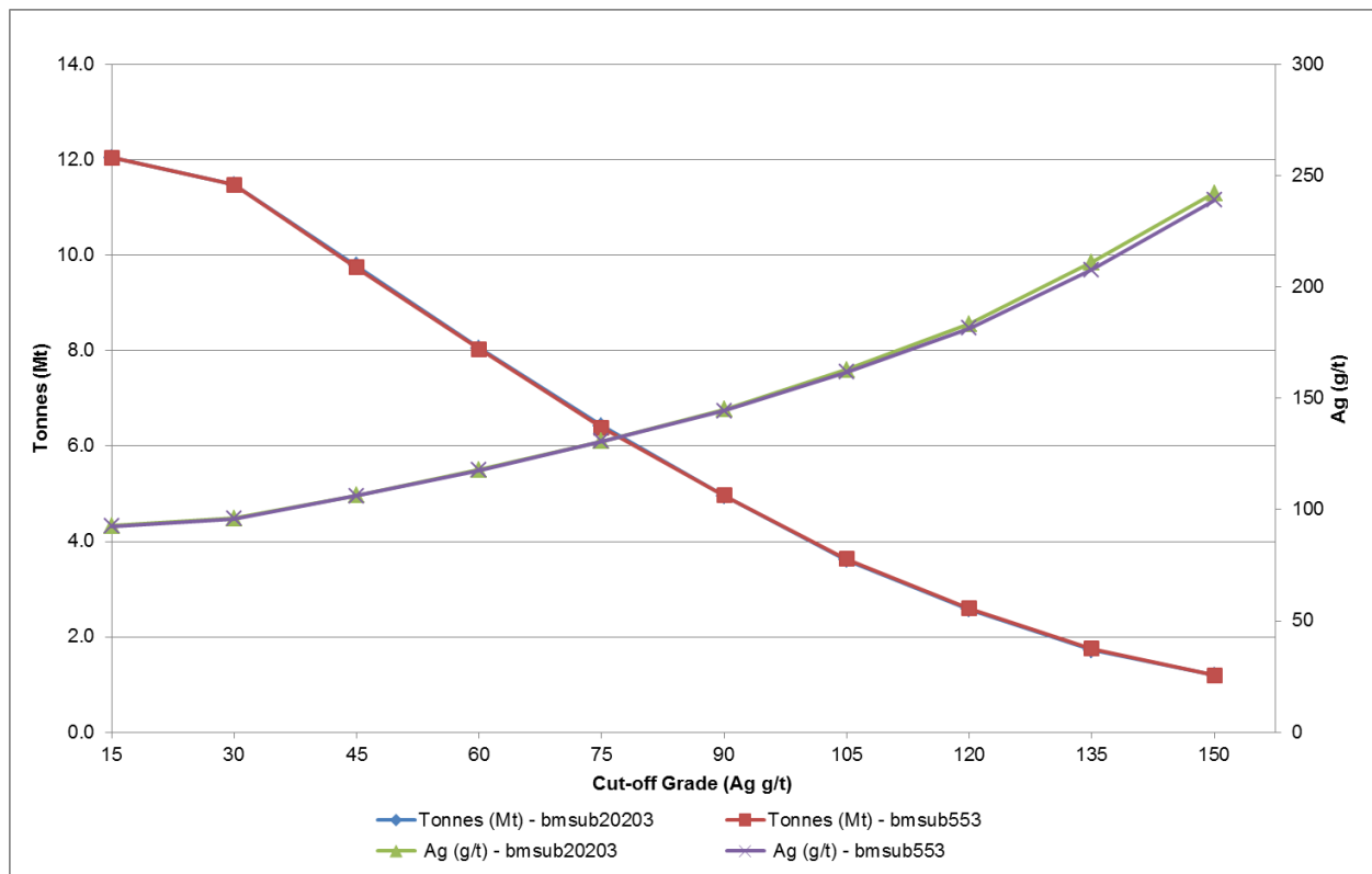
Figure 14-32 Grade-tonnage curves by parent block size
