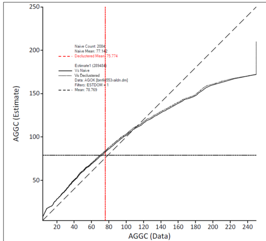
Figure 14-25 Q-Q plot: Domain I
