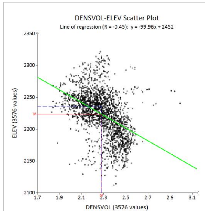
Figure I4-15 Scatterplot: Elevation versus Bulk density
