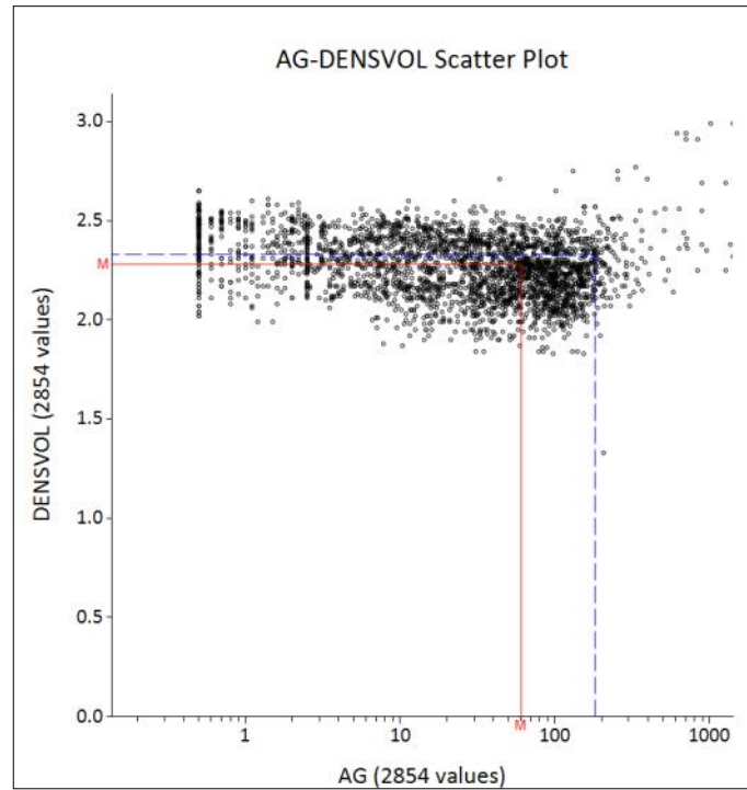
Figure I4-14 Scatterplot: Bulk density (dimension method) versus Silver grade
