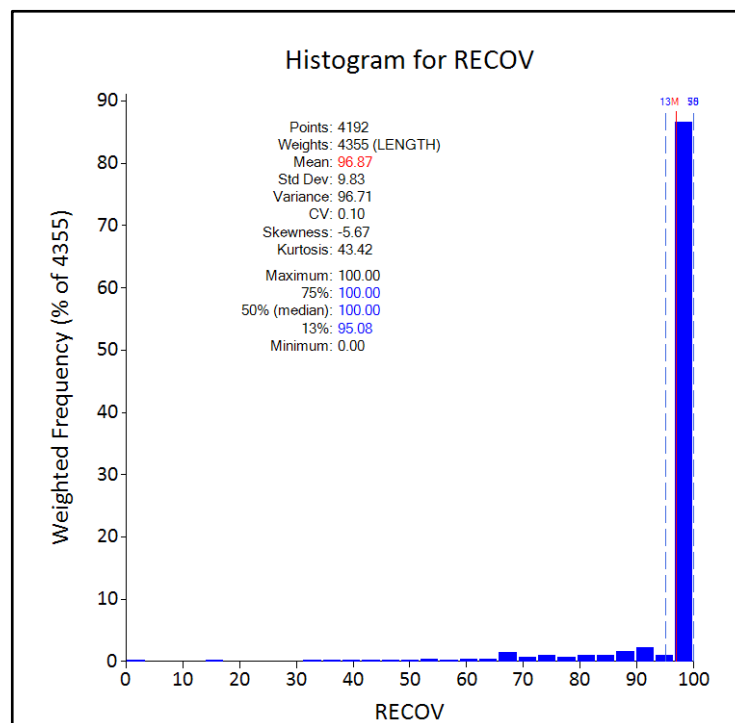
Figure 14-1 Drillhole recovery histogram
