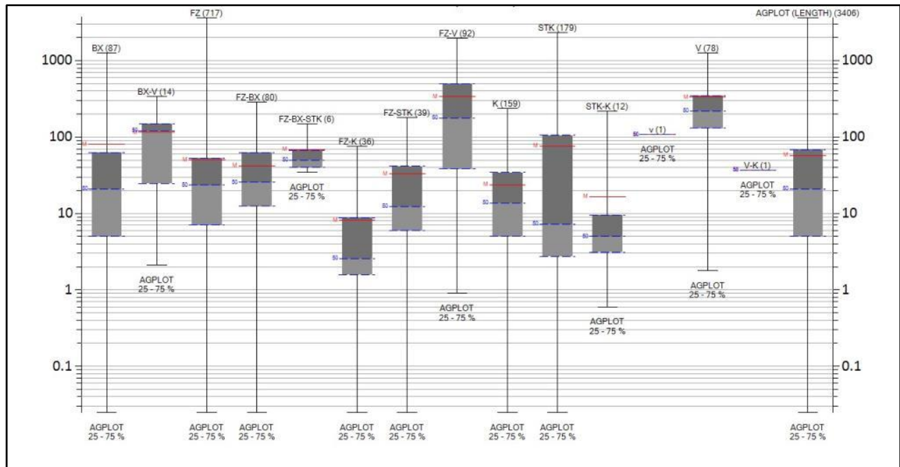
Figure 14-5 Silver box and whisker plot: Structural features
