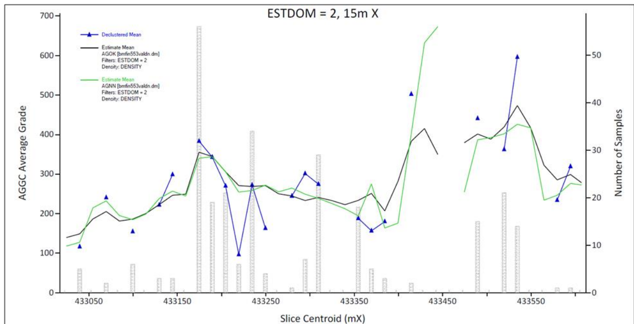
Figure 14-26 Swath plot: Domain 2 by Easting
