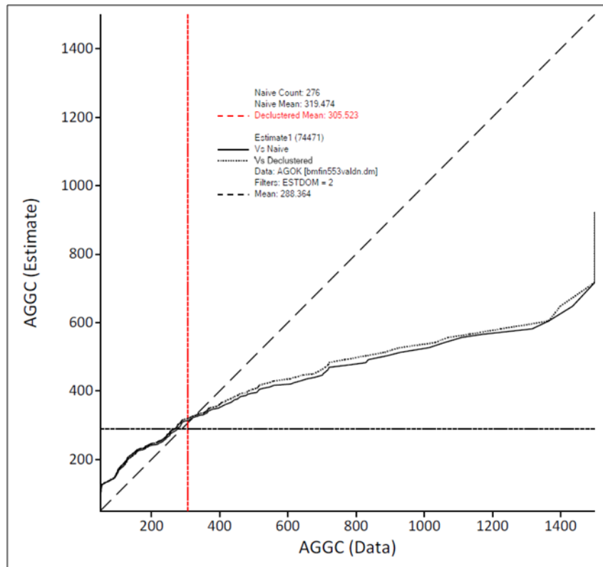
Figure 14-31 Q-Q plot: Domain 2
