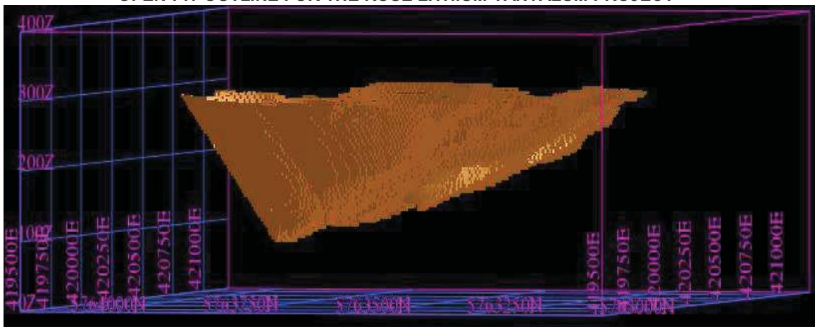
OPEN-PIT OUTLINE FOR THE ROSE LITHIUM-TANTALUM PROJECT
