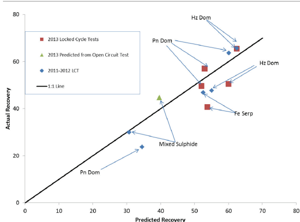
Figure 3: Locked Cycle Test Recovery Performance vs. Model
