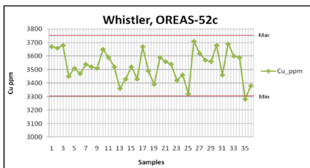
Figure 12-18 Standard Sample, OREAS-52c, Copper
