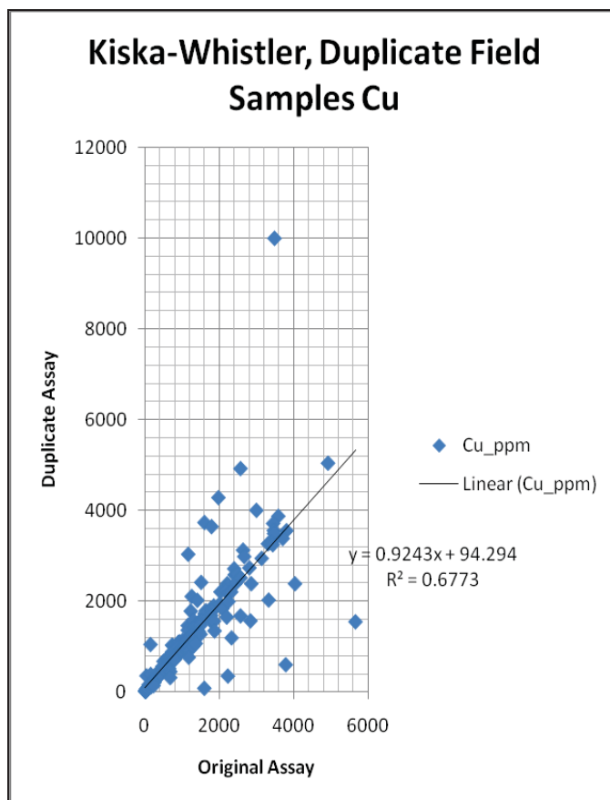
Figure 12-12 Duplicate Samples, Copper
