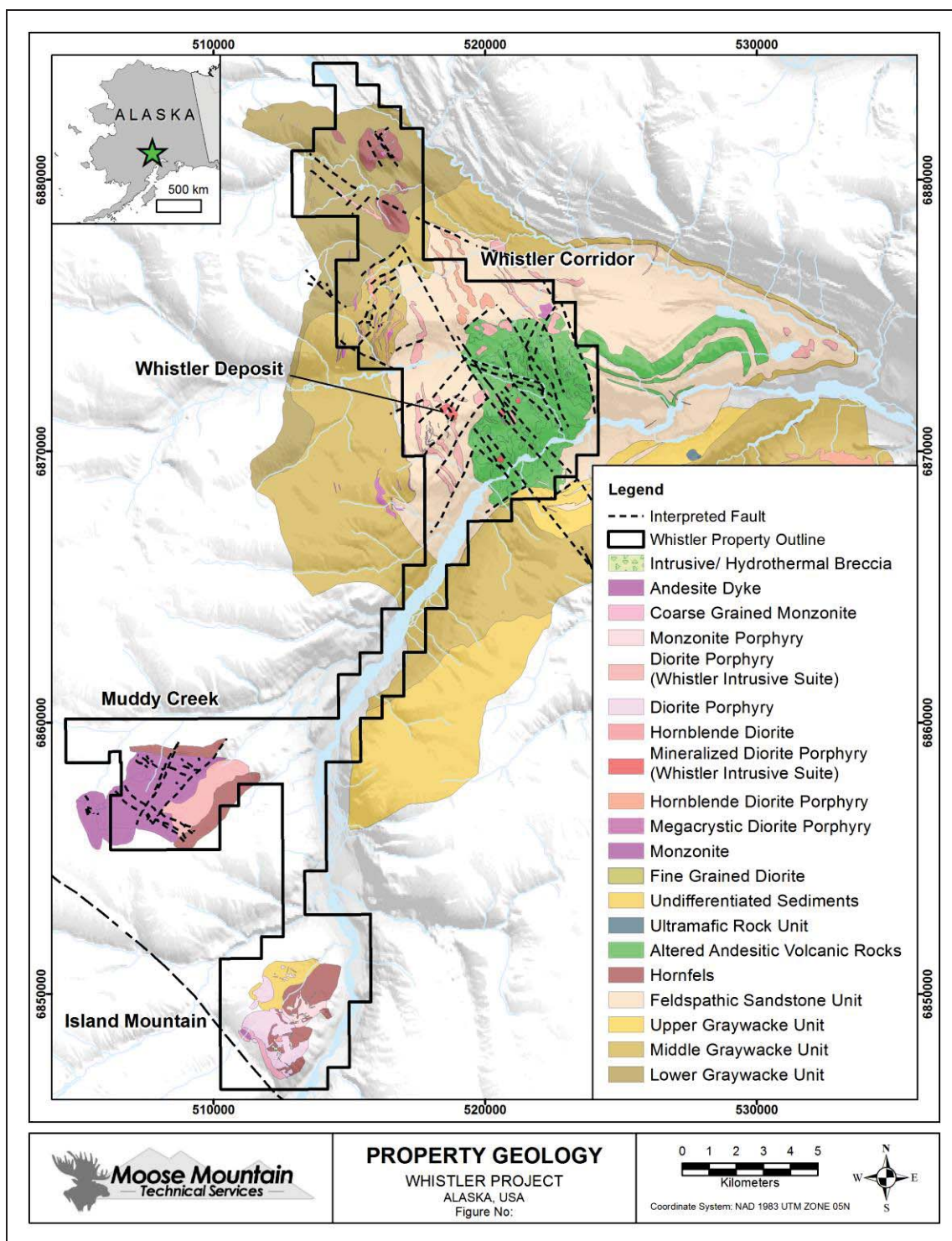
Figure 7-3 Geological Map of the Whistler Corridor (2015). Modified from Roberts, 2011a.
