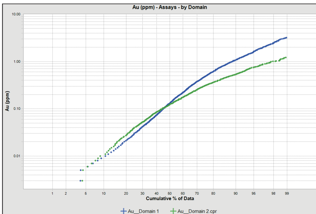
Figure 14-3 CPP of Au Assay Data by Domain
