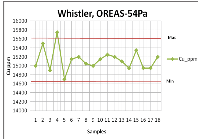
Figure 12-14 Standard Sample, OREAS-54Pa, Copper
