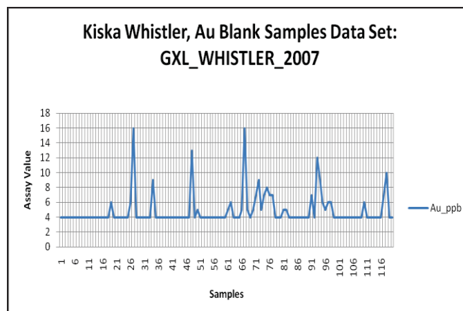
Figure 12-1 2007 Blank Samples, Gold
