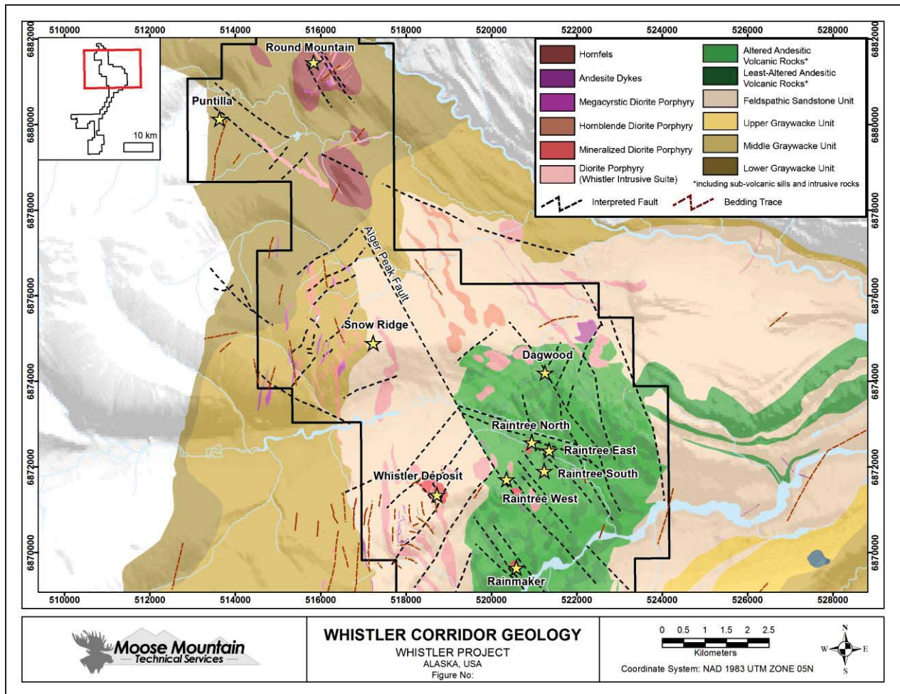
Figure 7-4 Whistler Project Geology (2015). Modified from Roberts, 2011a.
