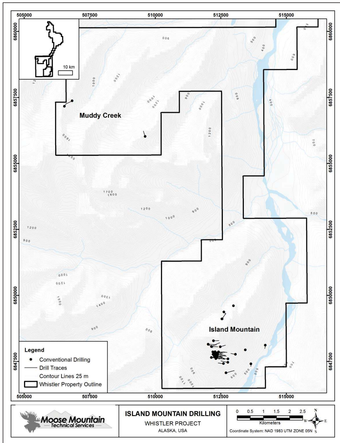
Figure 10-2 Island Mountain and Muddy Creek Drilling (2015)
