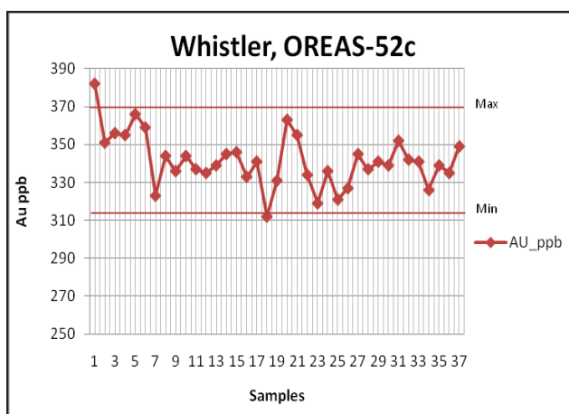
Figure 12-17 Standard Sample, OREAS-52c, Gold
