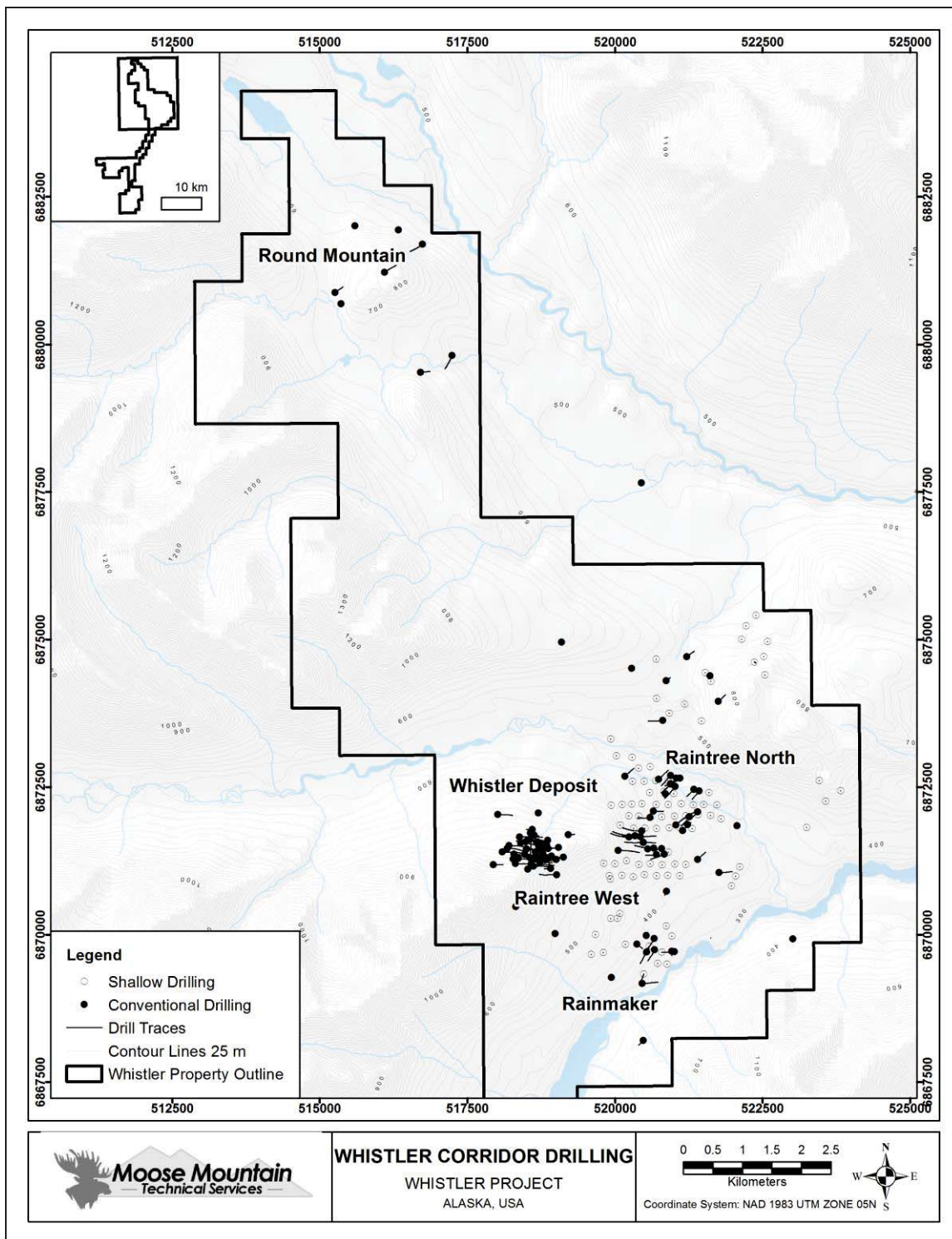
Figure 10-1 Whistler Area Drilling (2015)
