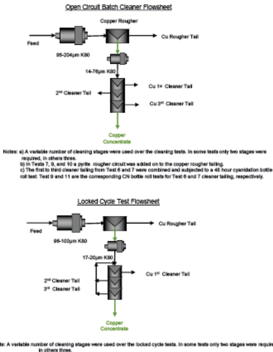
FIGURE 1 FLOTATION AND CYANIDATION FLOWSHEET AND TEST CONDITIONS
