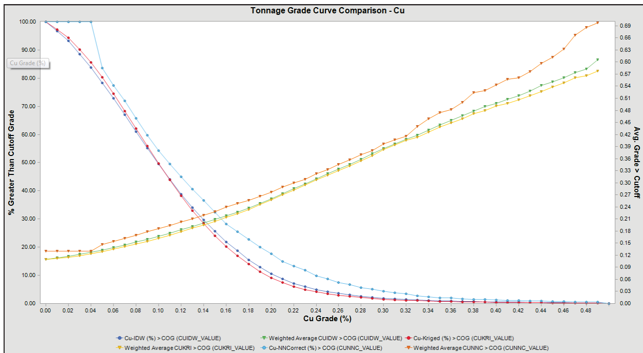
Figure 14-9 Tonnage-Grade Curves for Cu – Comparison of Interpolation Methods
