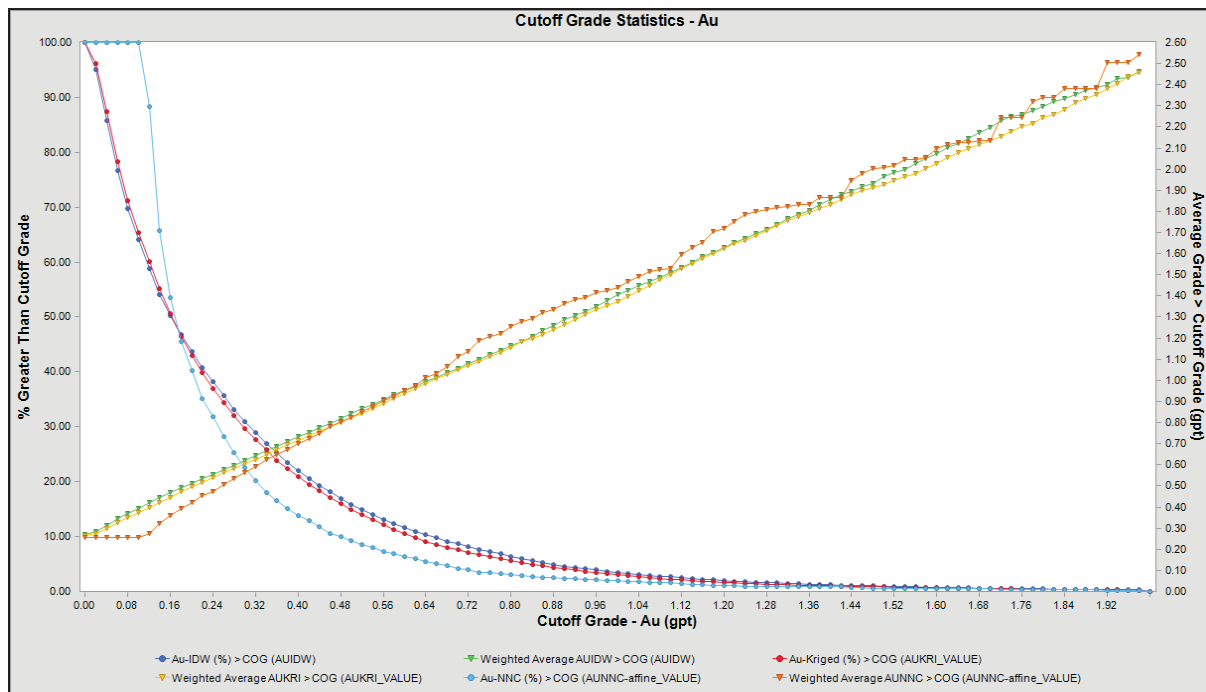
Figure 14-8 Tonnage-Grade Curves for Au – Comparison of Interpolation Methods
