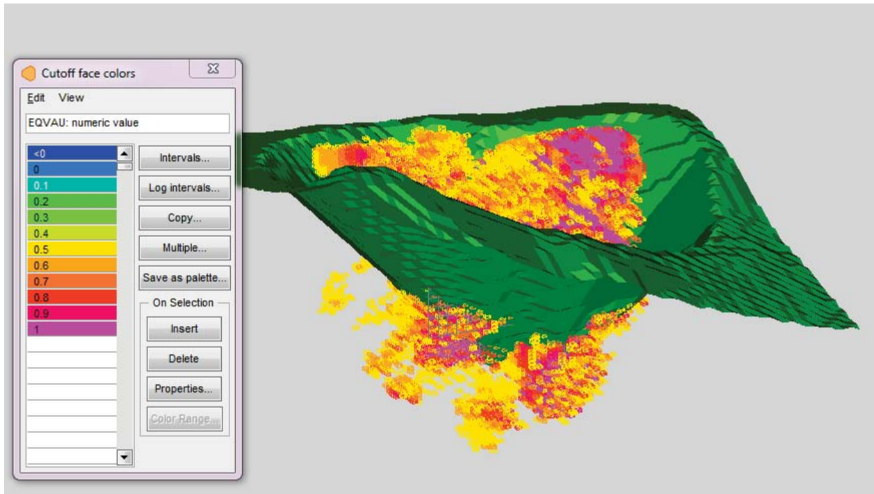
Figure 14-19 3D View looking N25E– Modelled Blocks within and Adjacent to Base Case Pit above a 0.5 gpt Au Eqv. Cut-off
