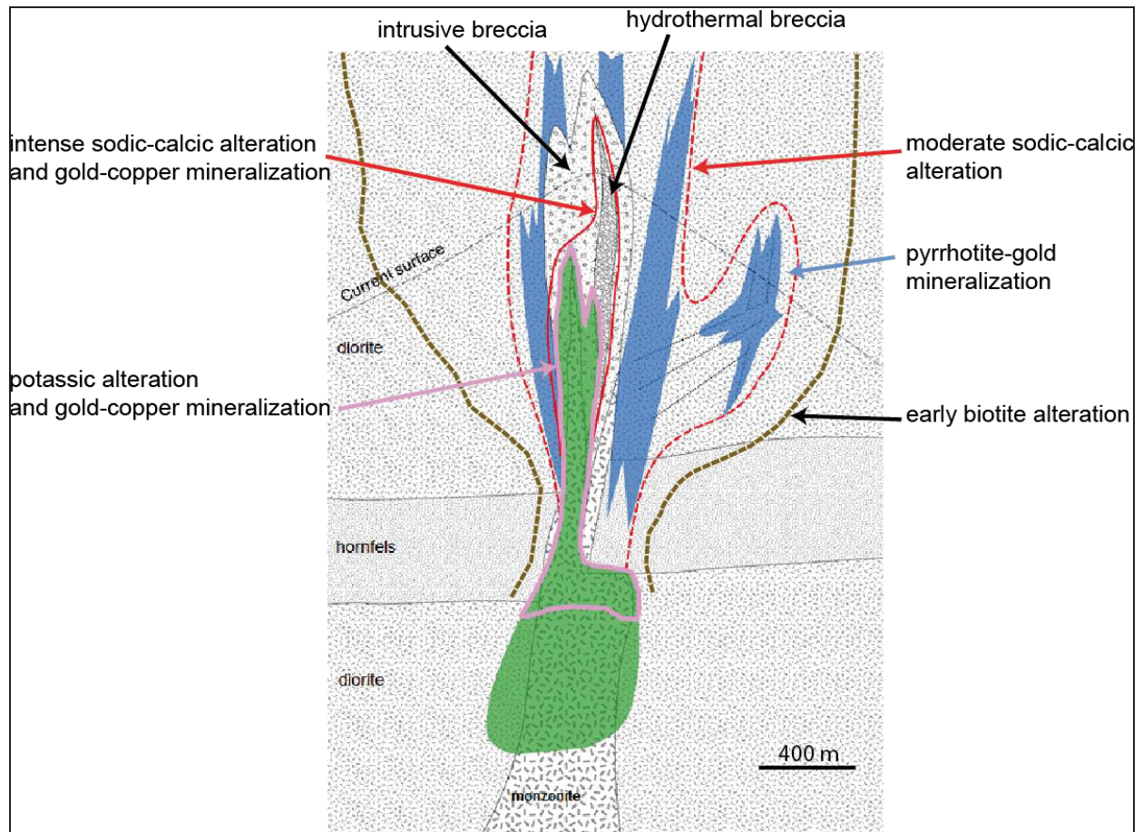
Figure 7-24 Schematic Model of Breccia Zone Alteration and Mineralization. From Roberts, 2011b.
