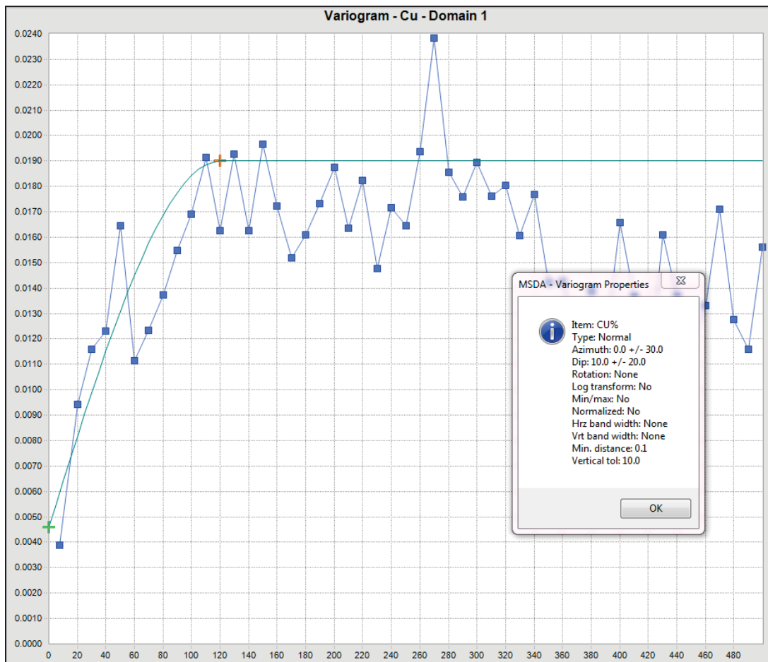
Figure 14-7 Variogram Model for Cu in Domain 1 – Major Axis
