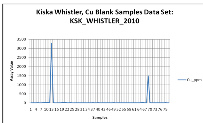
Figure 12-9 2010 Blank Samples, Copper
