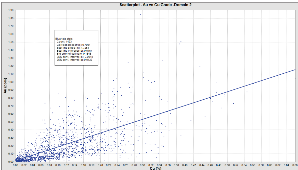
Figure 14-6 Scatter-plot of Au vs. Cu Grades – Domain 2
