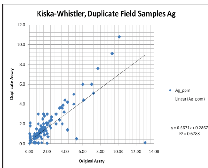
Figure 12-11 Duplicate Samples, Silver
