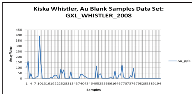
Figure 12-4 2008 Blank Samples, Gold
