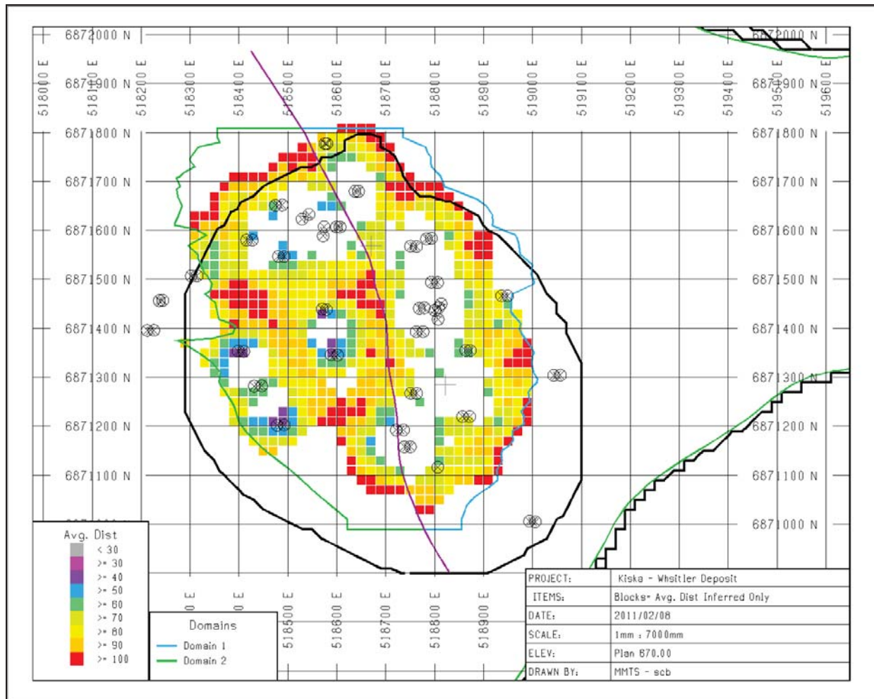
Figure 26-3 Plan of Average Distance to Composite for Inferred Blocks
