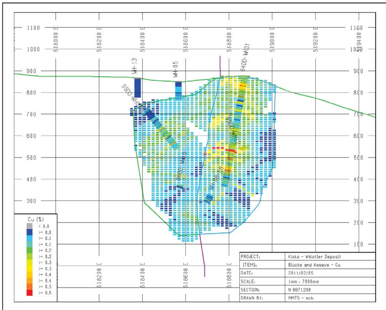
Figure 14-14 E-W Section Comparing Cu Grades for Block Model and Assay Data
