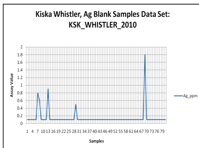
Figure 12-8 2010 Blank Samples, Silver
