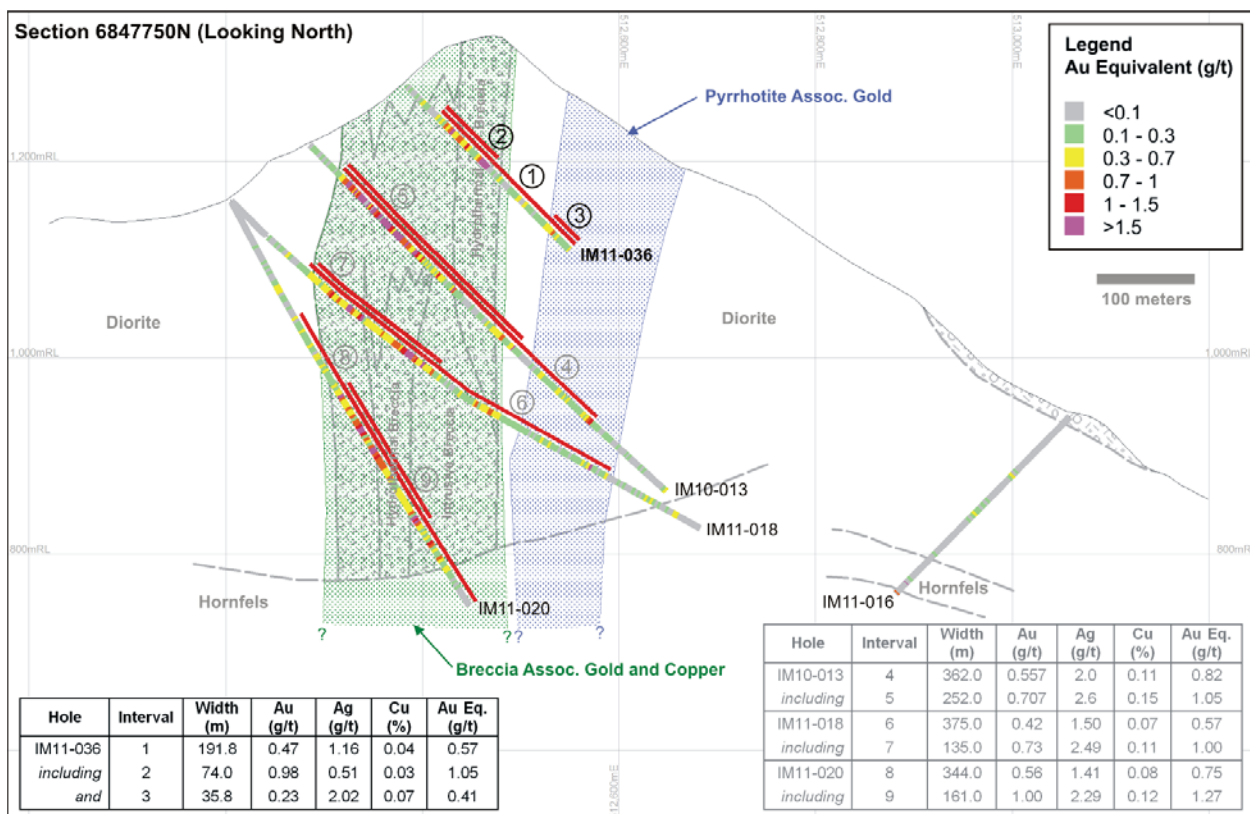
Figure 10-4 Cross-section 6847750N at the Island Mountain Breccia Zone. From Roberts, 2011b.
