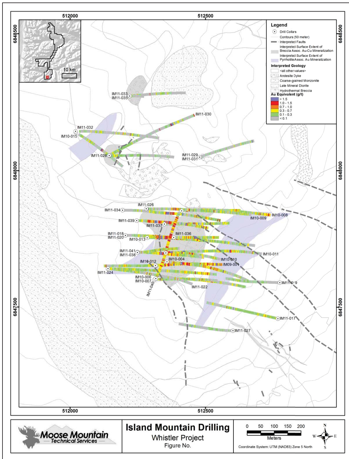
Figure 10-3 Plan Map of Drillholes and Mineralization Style at the Breccia Zone (2015). Modified from Roberts, 2011b.
