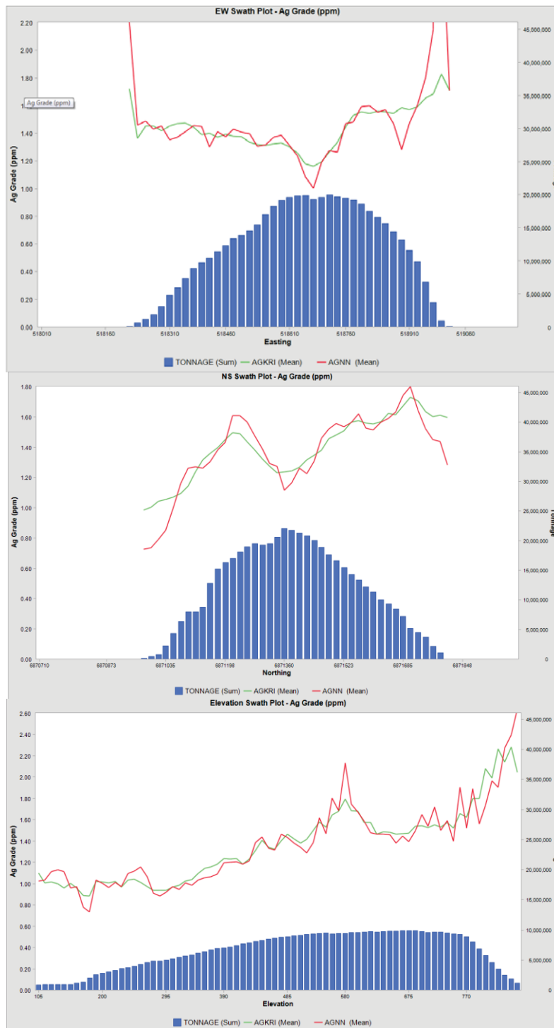
Figure 14-12 Swath Plots of Ag Grade
