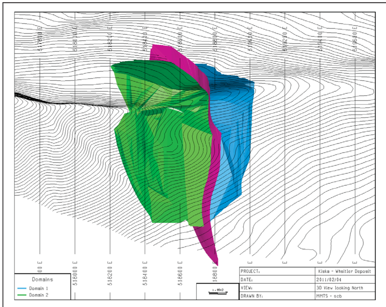
Figure 14-2 Divide Fault and Domains Modeled from Drillhole Geology
