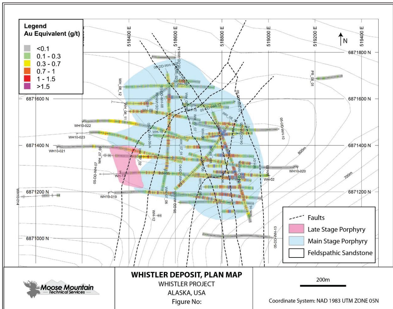
Figure 7-14 Geological Map of the Whistler Deposit (2015). Modified from AMC, 2012.
