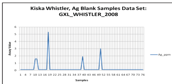
Figure 12-5 2008 Blank Samples, Silver
