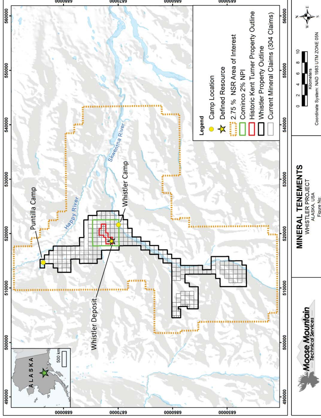
Figure 4-2 Tenement Map (2015). Modified from Roberts, 2011a.
