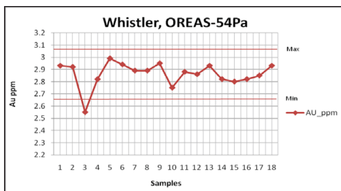
Figure 12-13 Standard Sample, OREAS-54Pa, Gold
