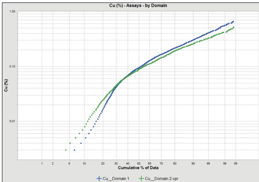
Figure 14-4 CPP of Cu Assay Data by Domain
