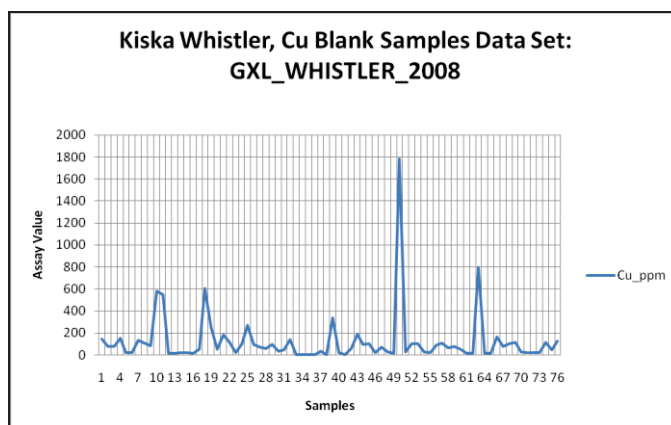
Figure 12-6 2008 Blank Samples, Copper
