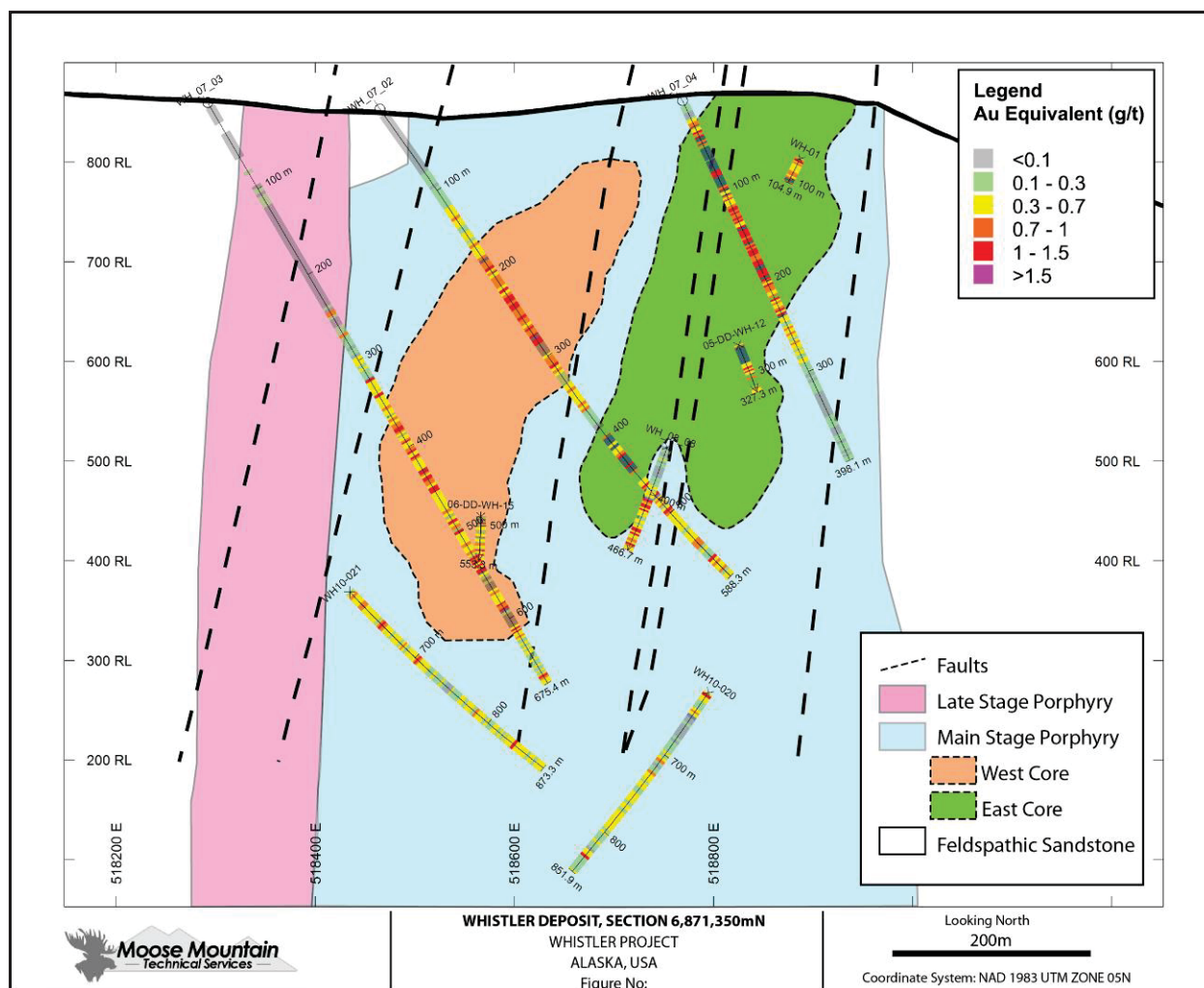
Figure 7-15 Geological Cross-section (6,871,350mN) of the Whistler Deposit (2015). Modified from AMC, 2012.
