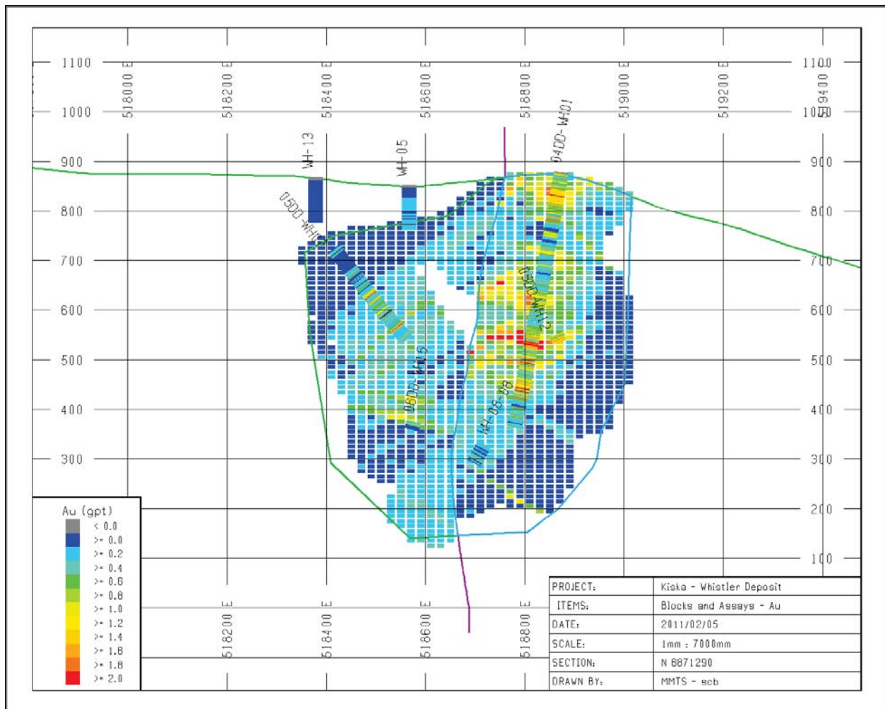
Figure 14-13 E-W Section Comparing Au Grades for Block Model and Assay Data
