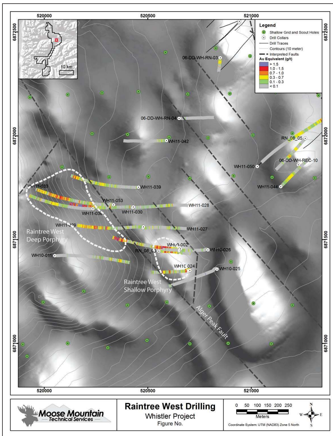
Figure 7-21 Plan Map of the Raintree West Prospect on a Background of greyscale airborne magnetic data, (magnetic high anomalies shown as lighter shades of grey) (2015). Modified from Roberts, 2011a.
