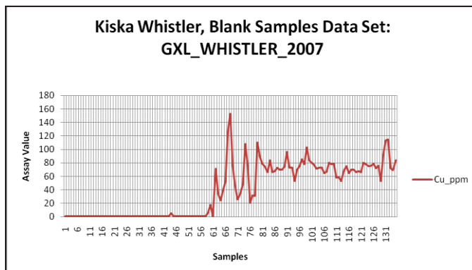
Figure 12-3 2007 Blank Samples, Copper
