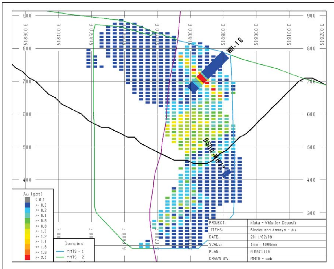
Figure 26-2 Section of Au Grade and Drilling at 6871110N
