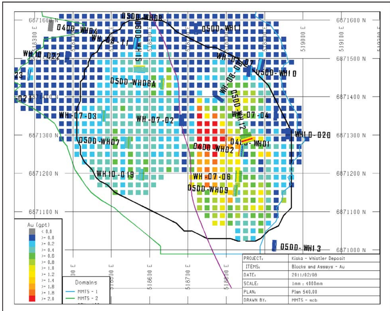
Figure 26-1 Plan of Au Grade and Drilling at 540m Elevation
