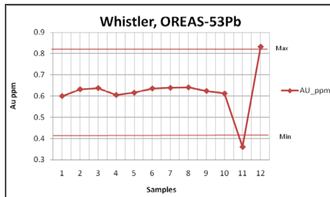
Figure 12-15 Standard Sample, OREAS-53Pb, Gold
