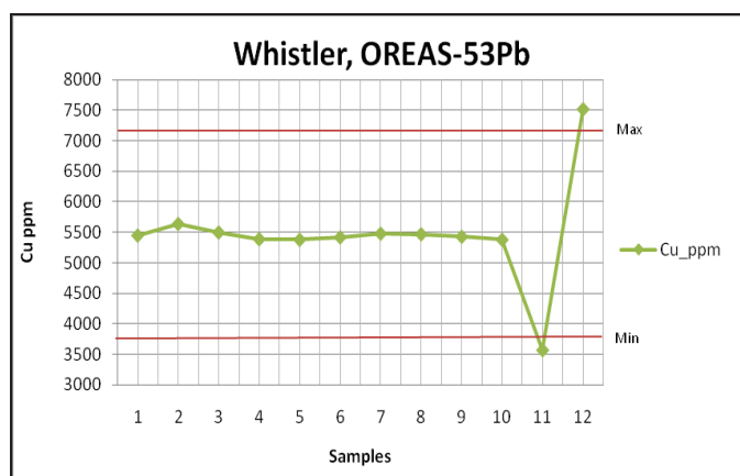
Figure 12-16 Standard Sample, OREAS-53Pb, Copper
