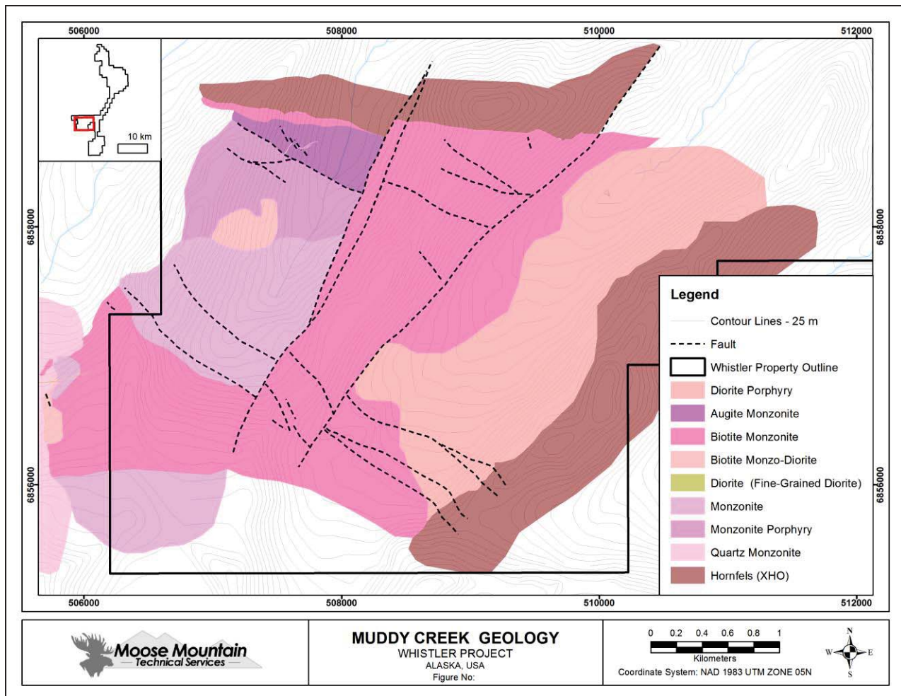
Figure 7-6 Geological Map of Muddy Creek (2015). Modified from Roberts, 2011c.
