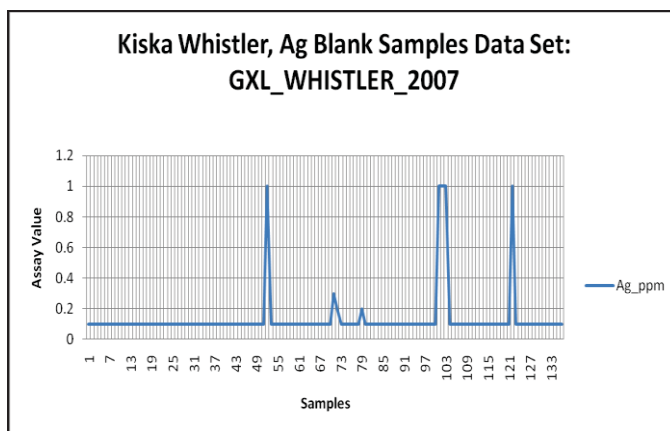
Figure 12-2 2007, Silver Blank Samples
