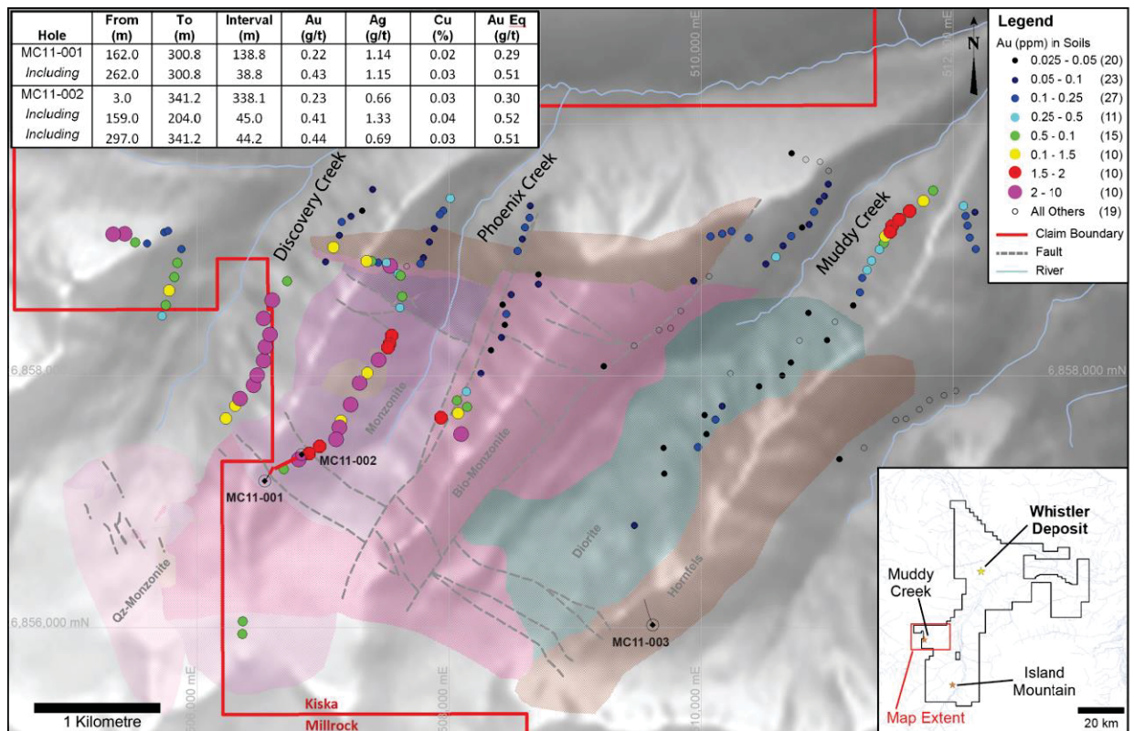
Figure 10-5 Plan Map of 2011 Muddy Creek Drilling with Geology and Au Soil Geochemistry. From Roberts, 2011c.
