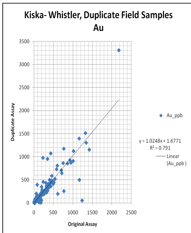
Figure 12-10 Duplicate Samples, Gold
