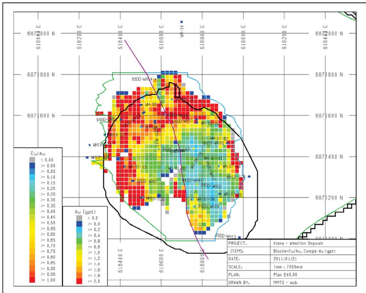
Figure 14-18 Plan of the Cu/Au Ratio Indicating Spatial Variability
