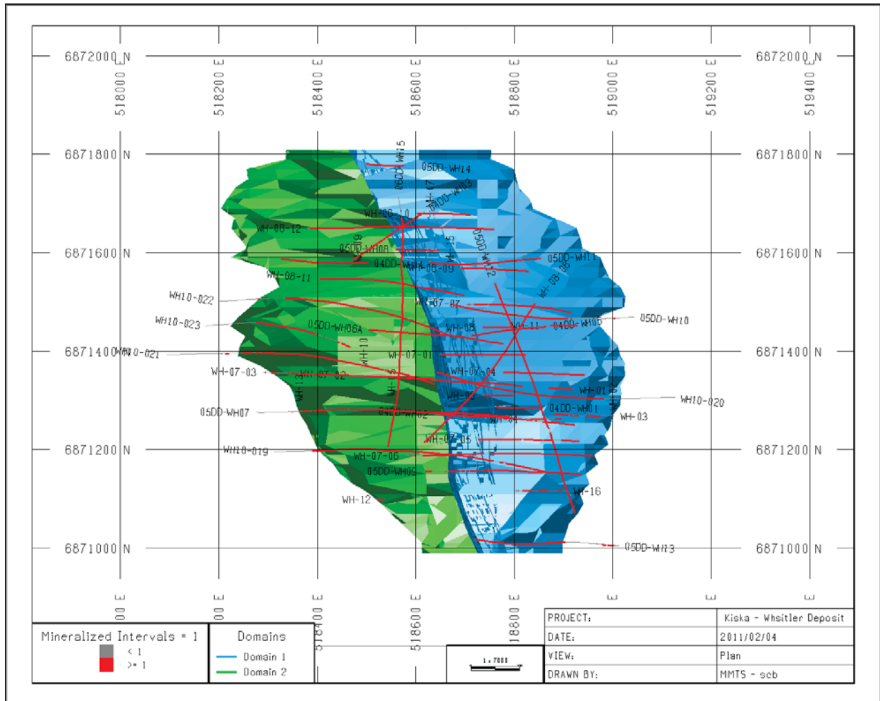
Figure 14-1 Plan view of the Mineralized Assay Intervals and Domains of the Diorite Solid
