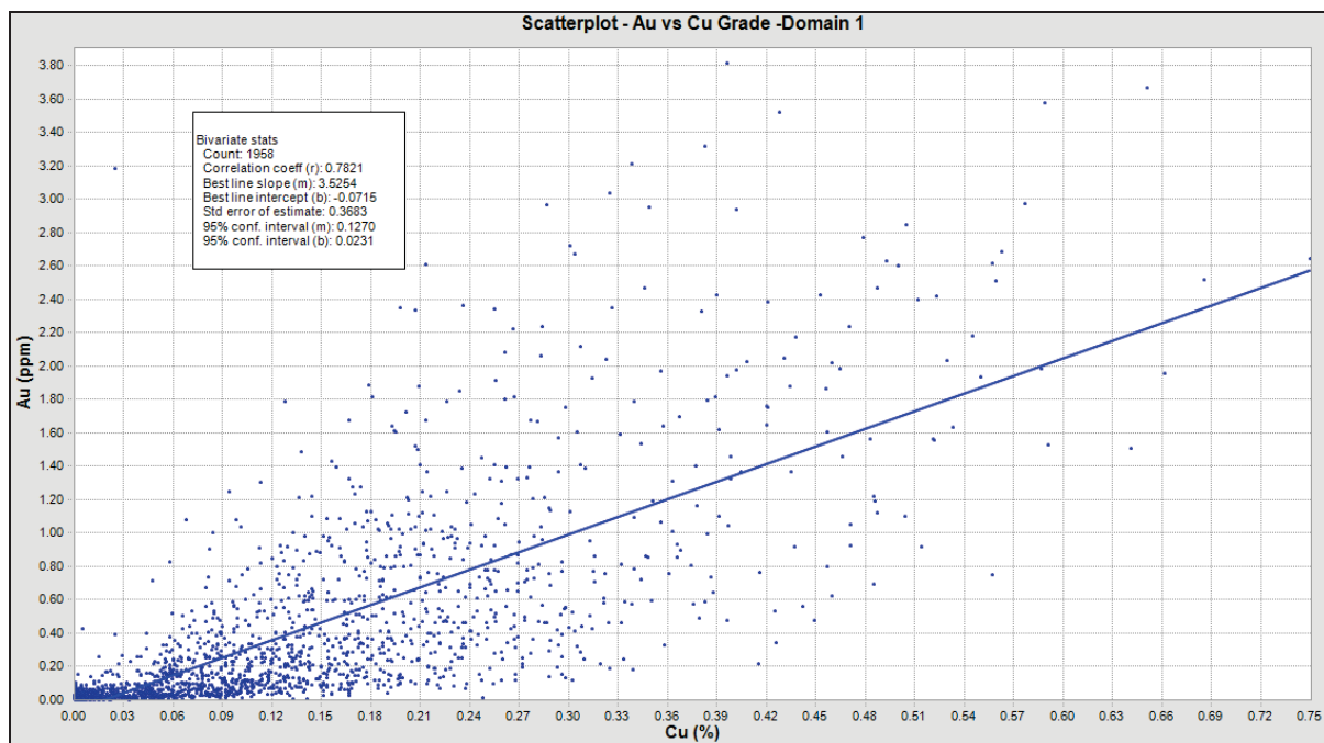
Figure 14-5 Scatter-plot of Au vs. Cu Grades – Domain 1
