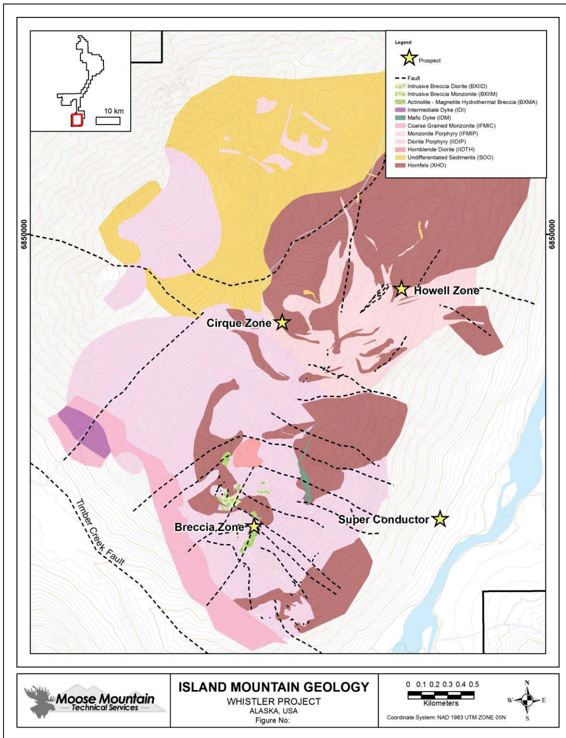
Figure 7-5 Property Geology of the Island Mountain Area (2015). Modified from Roberts, 2011b.
