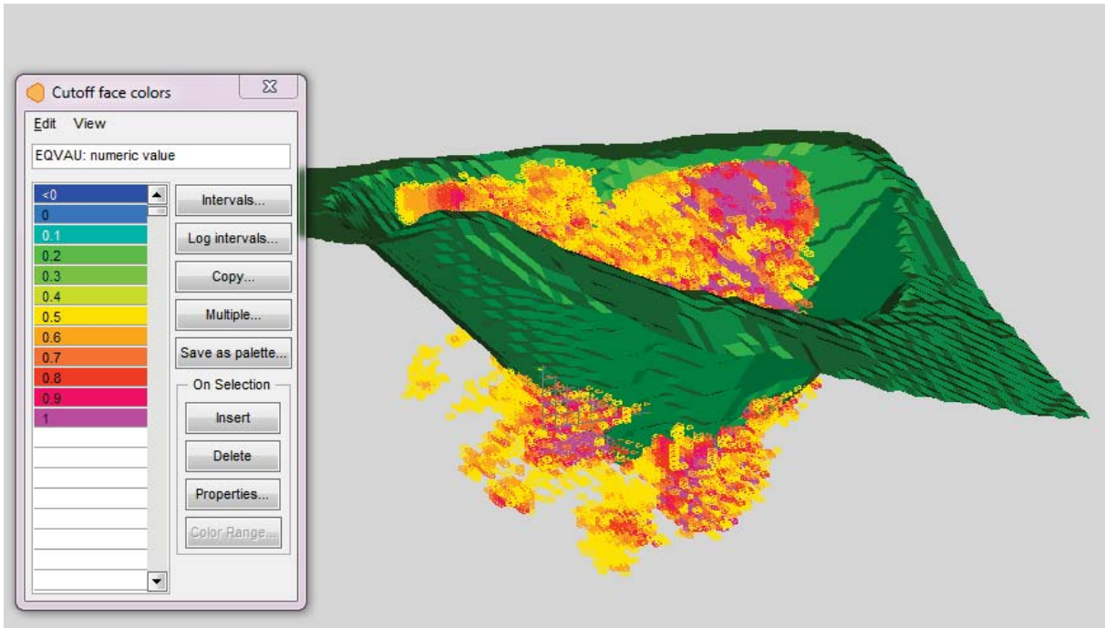
Figure 1-1 3D View looking N25E– Modelled Blocks within and Adjacent to Base Case Pit above a 0.5 gpt Au Eqv. Cut-off
